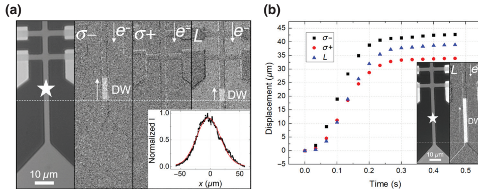
FIG. 2. (a) Kerr images of a 4\text{-}\mu\text{m} Co/Ni/Co ferromagnetic wire. Linear ( L ), right-circularly ( \sigma^+ ), and left-circularly ( \sigma^- ) polarized laser beams shine on the sample with a fluence of 4 \text{ mJ/cm}^2 for 10 \text{ s} , together with synchronized current pulses of 7.3 \times 10^6 \text{ A/cm}^2 and 10\text{-}\mu\text{s} pulse duration ( 5\text{-kHz} -repetition rate), both of which are below the threshold value for domain-wall motion. Inset: Gaussian profile of the laser spot with a FWHM of 47 \mu\text{m} . (b) Time evolution of the domain-wall displacement of a 4\text{-}\mu\text{m} Co/Ni/Co ferromagnetic wire from domain-wall video recording and analysis with the APREX TRACK software as a function of the laser polarization, where the current density is increased to 14.6 \times 10^6 \text{ A/cm}^2 . Inset: Kerr images of a 4\text{-}\mu\text{m} Co/Ni/Co ferromagnetic wire, which shows the domain-wall motion with a Linear ( L ) laser beam. The initial magnetization saturation direction is M \uparrow and the white contrast corresponds to a reversal to M \downarrow .
