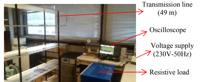
Figure 5. Experimental test bench.
