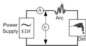
Fig. 8: Drill in series with an arc fault.
