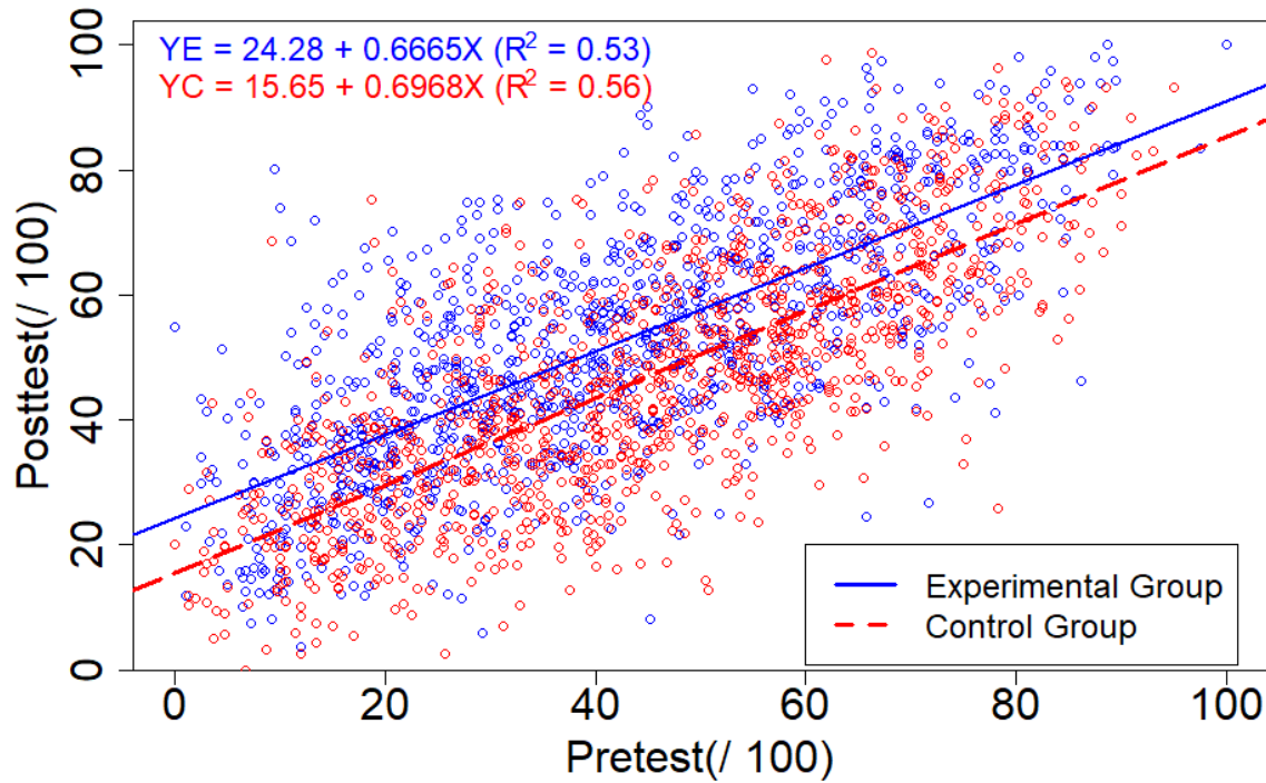
Figure 3. Scatter diagram for composite scores on the pretest and the posttest for the whole sample of 2295 students, with regression lines and equations for the two sub-groups.
