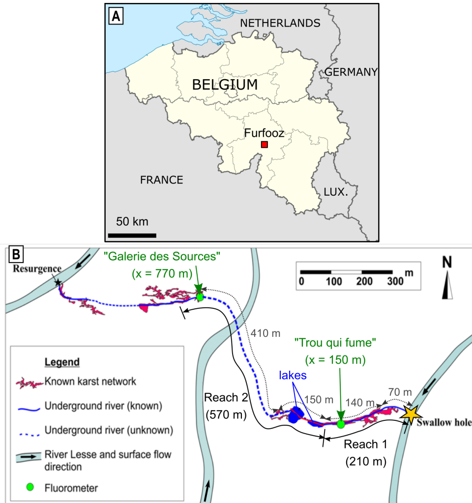
Figure 8 The Furfooz karstic system and its numerical representation. Two sampling locations are considered : the Trou qui fume and the Galerie des Sources . The system is approximated by two reaches: (i) the first one represents a first mainly advective part ; (ii) the second reach represents the ensemble made by the lakes and their unexplored downstream part.
