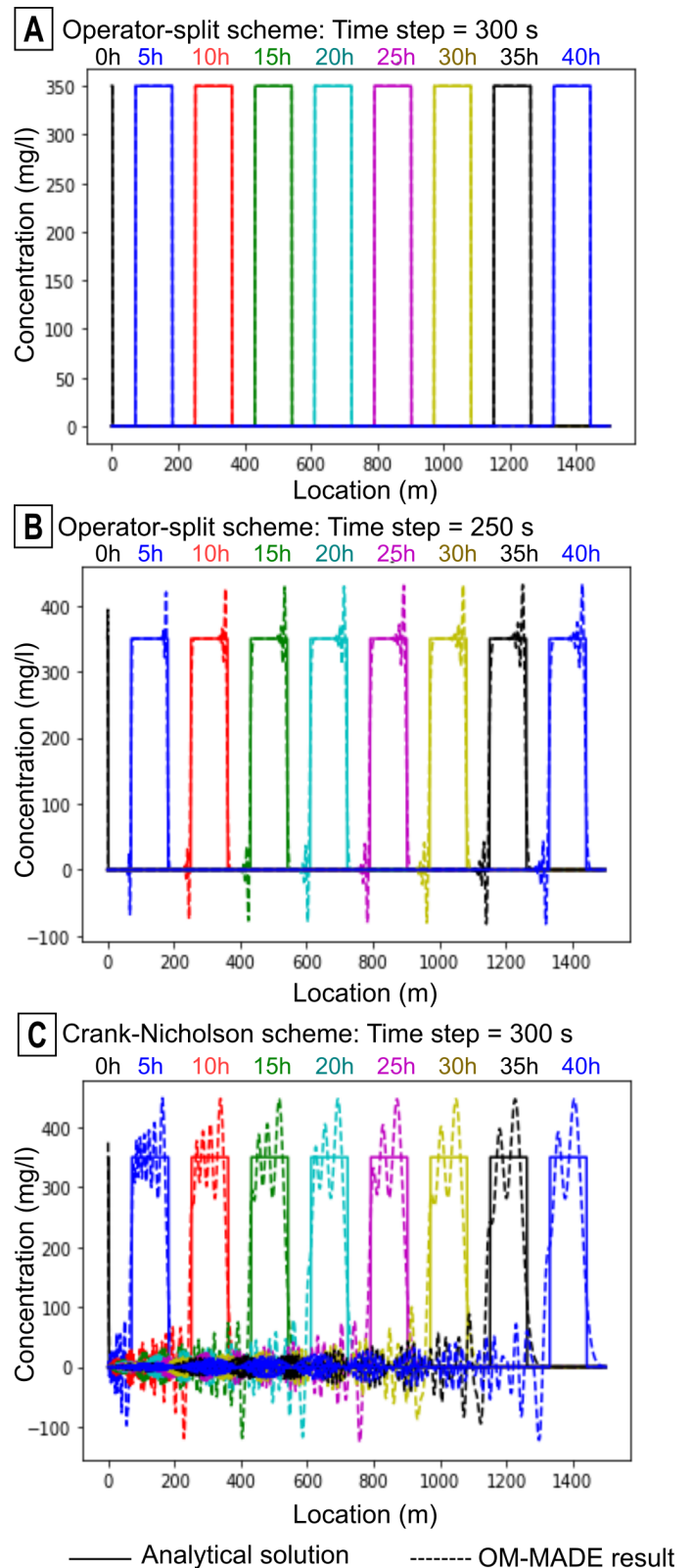
Figure 3 Comparison of OM-MADE results with an analytical solution in the case of a pure advective flow: the concentration profiles are plotted each 5 h along the conduit. In (A) and (B), OM-MADE uses the operator-split scheme (Lax-Wendroff scheme for advection resolution) with a time step of 300 s in (A) and 250 s in (B). In (C) OM-MADE is run using a Crank-Nicholson scheme and a time step of 300 s.
