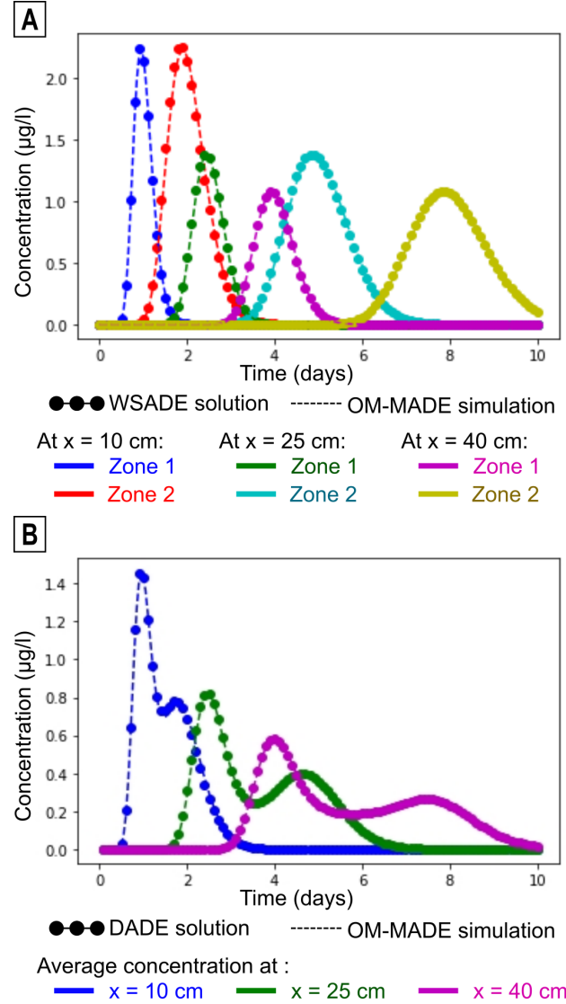
Figure 5 Simulation of two mobile zones and comparison with solutions of Field and Leij [2012] at three positions: (A) in the case where no exchange are allowed between the two zones (WSADE solution); (B) in the case where exchanges are taken into account between both zones (DADE solution)
