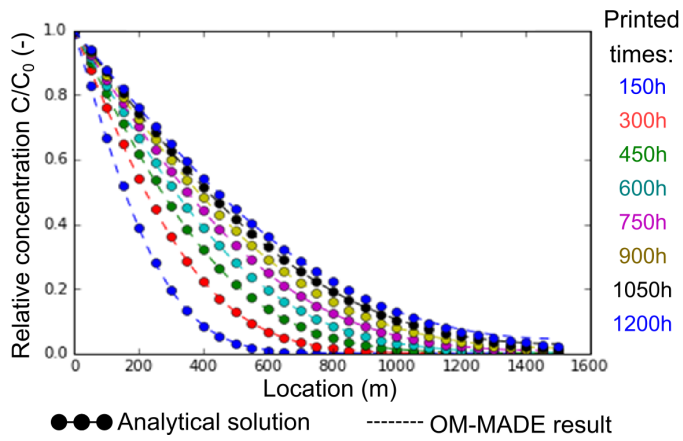
Figure 2 Comparison of OM-MADE result with an analytical solution in the case of a pure diffusive flow. At t = 1200h , the tracer arrives at the output location, thus the semi-infinite wall condition is no more valuable and explains the small differences that can be observed with the analytical solution.
