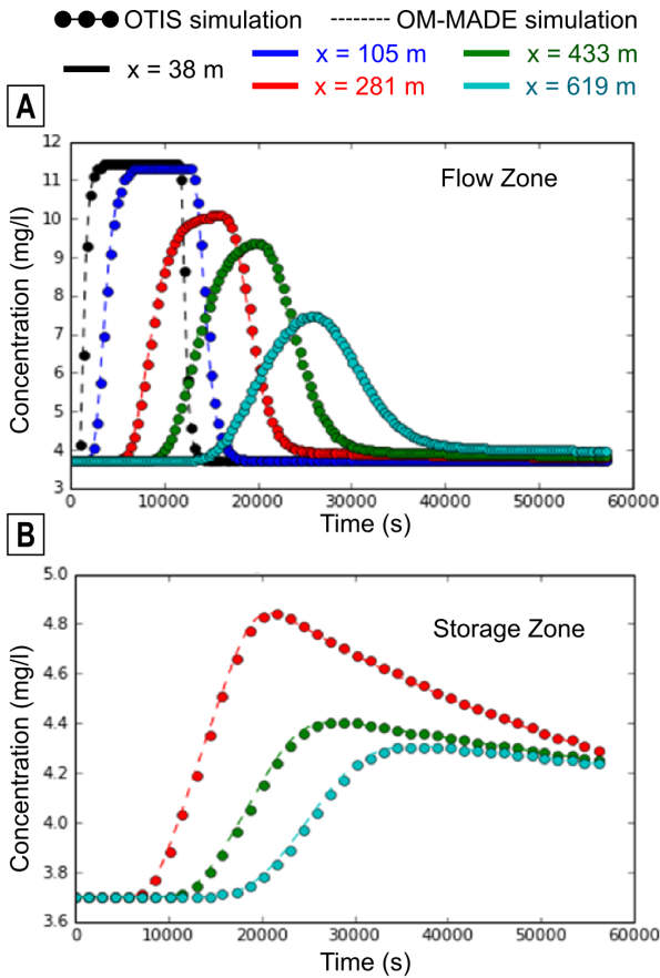
Figure 6 Simulation of BTCs in the case of multi-reach single flow with storage: the domain is divided in 5 reaches, one mobile zone exchanges with storage zones in the reaches 3, 4, and 5. Simulated concentrations with OTIS and OM-MADE: (A) in the flow zone and (B) in the storage zones.
