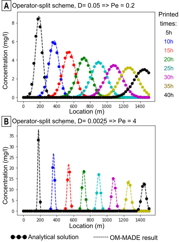
Figure 4 Comparison of OM-MADE results (operator-split scheme) with an analytical solution in the case of advective-dispersive flow. In (A) the hydrodynamic dispersion coefficient D = 0.05 \text{ m}^2/\text{s} which leads to Pe = 0.2 . In (B) D = 0.0025 \text{ m}^2/\text{s} which leads to Pe = 4 , a value often considered as the usability limit of second order schemes.
