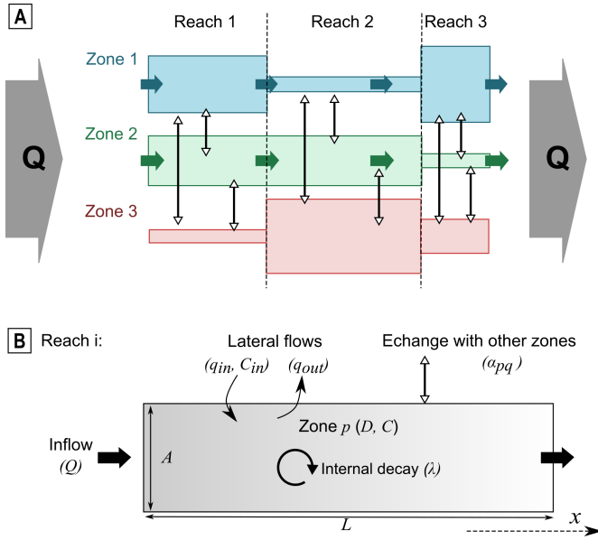
Figure 1 Schematic representation of an OM-MADE model: (A) In this example, two mobile zones (zone 1 and 2) are interconnected with one storage zone (zone 3). The total flowrate Q is preserved all along the flow (steady flow regime). Three reaches are defined to allow longitudinal variations of the system geometrical characteristics. (B) Detailed representation of one reach of a zone p : a reach is defined by a given length L , a cross-sectional area A , a dispersion coefficient D , a solute concentration C , linear lateral flows (in/out flowrates and concentration q_{in} , q_{out} , C_{in} ), internal decay (coefficient \lambda ) and exchange(s) with other(s) zone(s) (coefficient(s) \alpha_{pq} ).
