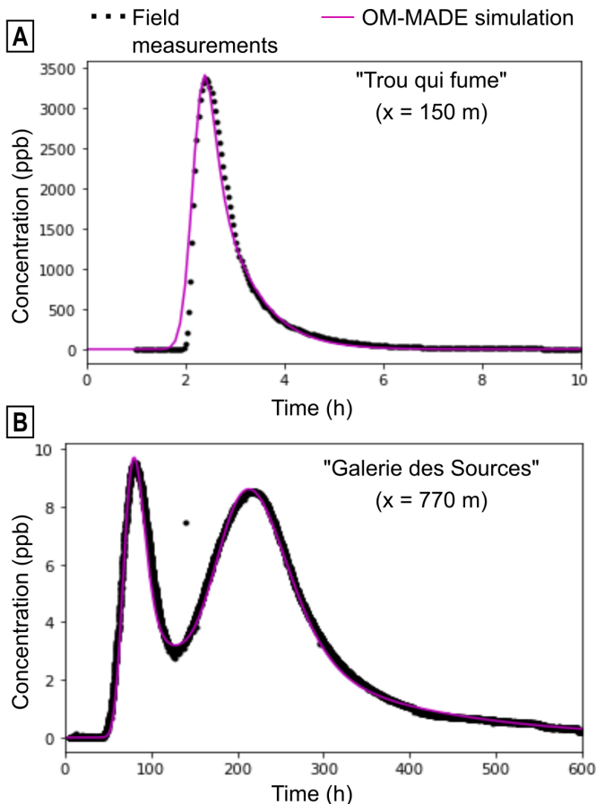
Figure 9 OM-MADE simulated BTC fit to a tracer test conducted in Furfooz. The first site, named "Trou qui fume" is located 150 m downstream the swallow hole while the second site, the "Galerie des Sources" is located 770 m downstream the injection point.
