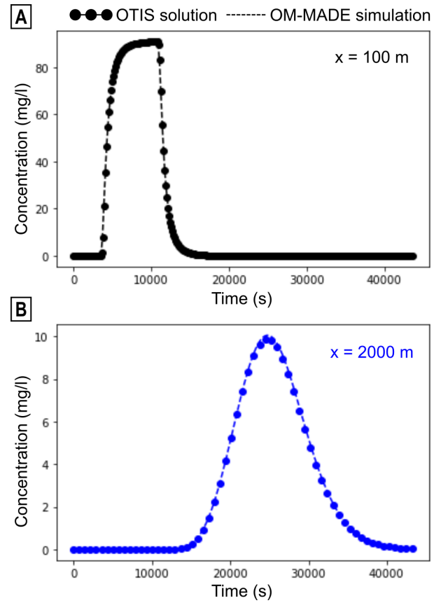
Figure 7 OM-MADE results compared to OTIS solution in the case of transport with first-order decay.
