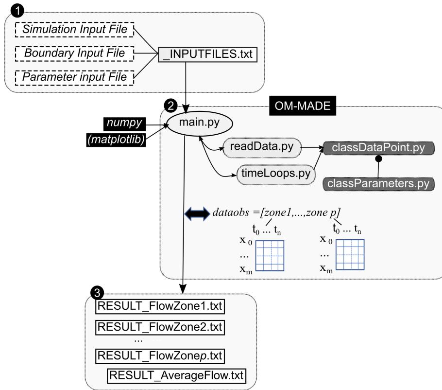
Figure 11 OM-MADE architecture: Three text input files are required by the _INPUTFILES.txt file (1). They contain all information to run a specific simulation. OM-MADE (2) should be launched by running the main program (several examples are provided), which calls four python modules. The result of a simulation is stored in the dataobs variable, which is a list of arrays containing, for each zone, the concentration for each printed time and distance. This variable can be used to generate several text files containing the result of the simulation (3).
