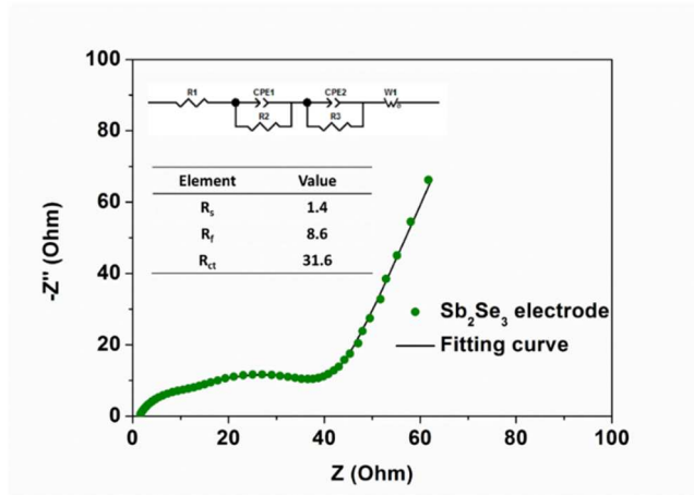
Fig. 6 EIS plot and the corresponding fitting curve of Sb_2Se_3 electrode (inset are the equivalent circuit and a summary of simulation results of resistance value).
