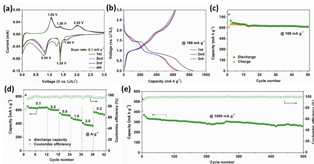
Fig. 5 Lithium storage performances of \text{Sb}_2\text{Se}_3 nanowires electrode: (a) Cyclic voltammogram curves at a scan rate of 0.1 \text{ mV s}^{-1} ; (b) first three charge-discharge profiles at a current density of 100 \text{ mA g}^{-1} ; (c) cycling performance at a current density of 100 \text{ mA g}^{-1} ; (d) rate performances at various current densities; (e) long-term cycling performance at a current density of 1000 \text{ mA g}^{-1} .
