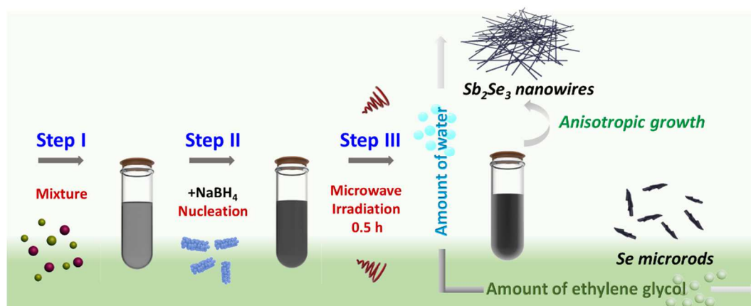
Fig. 4 Schematic illustration of synthesis procedure and formation mechanism of Sb 2 Se 3 nanowire via solvent-mediated microwave irradiation.
