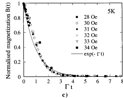
FIG. 7. Variation of the reduced magnetization B as a function of \Gamma t collected from a GdFe(1000 Å)/TbFe(3 Å)/GdFe(500 Å) sample under different magnetic fields (a) at 3 K, (b) at 4 K, (c) at 5 K. The \Gamma values are reported in Table I.
