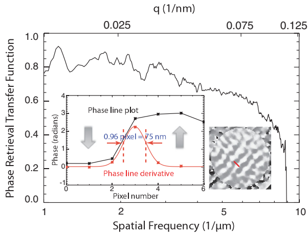
FIG. 3 (color). The Wiener-filtered phase retrieval transfer function [16] of the reconstruction in Fig. 2. This is the ratio of the magnitude of the complex amplitude with the square root of the measured intensity. Inset: a plot across the domains of the phase-only image, along with arrows showing orientation of the domains. The derivative is given by the red curve and gives an estimated resolution of about 75 nm.
