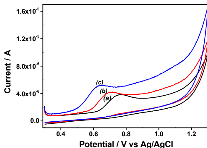
Fig. 1. Cyclic voltammograms of 100 \mu M DCF at the GCE ( a , black), GCE/AT ( b , red) and GCE/Amino-AT ( c , blue) in 0.1 M NaCl pH 6. The scan rate was 50 mV·s -1 .
