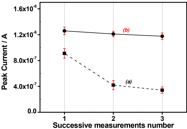
Fig. 9. SWV responses recorded in triplicate with (a) GCE/Amino-AT and (b) GCE/APTES-Amino-AT-Silica to successive preconcentration/detection of 5 \mu M DCF in phosphate buffer pH 5.7 after 2 min accumulation. A step of cleaning the surface of the modified electrode between each successive measurement has been applied under stirring for 15 min in (a) 0.1 M HCl and (b) ethanol solution (to remove the adsorbed DCF oxidation products).
