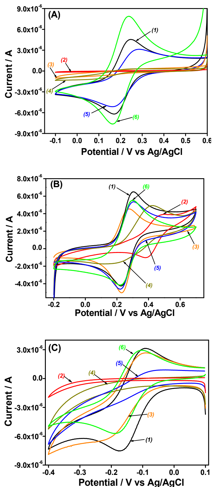
Fig. 4. Cyclic voltammograms recorded in 0.1 M \text{NaNO}_3 containing (A) 0.5 mM [\text{Fe}(\text{CN})_6]^{3-} , (B) 0.5 mM \text{Fc}(\text{MeOH})_2 and (C) 0.5 mM [\text{Ru}(\text{NH}_3)_6]^{3+} , using various electrodes: (1) bare GCE; (2,3) GCE/APTES-Silica before (2) and after surfactant removal (3); (4,5) GCE/APTES-Amino-AT-Silica before (4) and after surfactant removal (5); (6) GCE/Amino-AT. The potential scan rate was 50 \text{ mV s}^{-1} in all cases.
