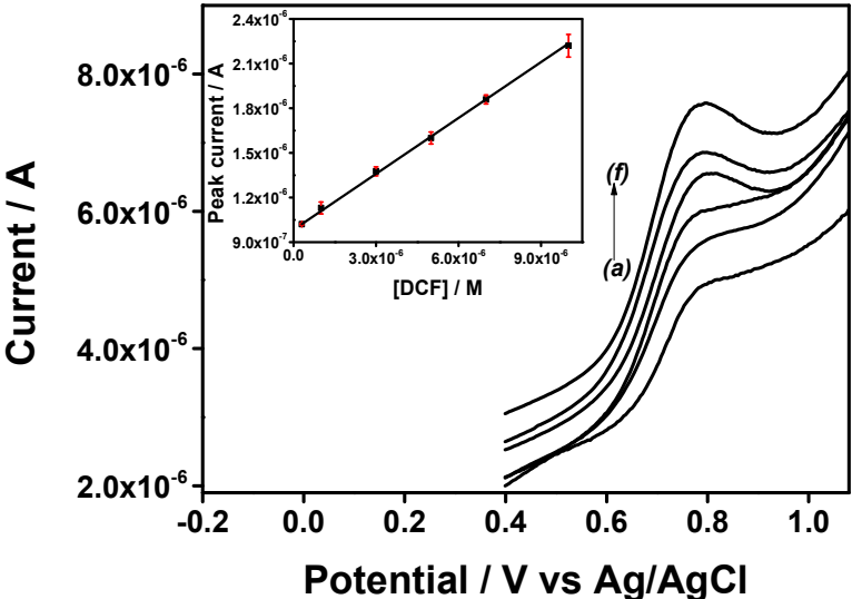
Fig. 8. Square-wave voltammograms recorded for DCF in phosphate buffer pH 5.7, in the 0.3 to 10 \mu M concentration range, using GCE/APTES-Amino-AT-Silica electrode. Inset: corresponding calibration curve obtained from SWV curves recorded in triplicates. Accumulation time: 3 min.
