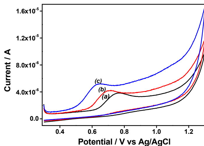
Fig. 1. Cyclic voltammograms of 100 \mu M DCF at the GCE ( a , black), GCE/AT ( b , red) and GCE/Amino-AT ( c , blue) in 0.1 M NaCl pH 6. The scan rate was 50 mV \cdot s^{-1} .
