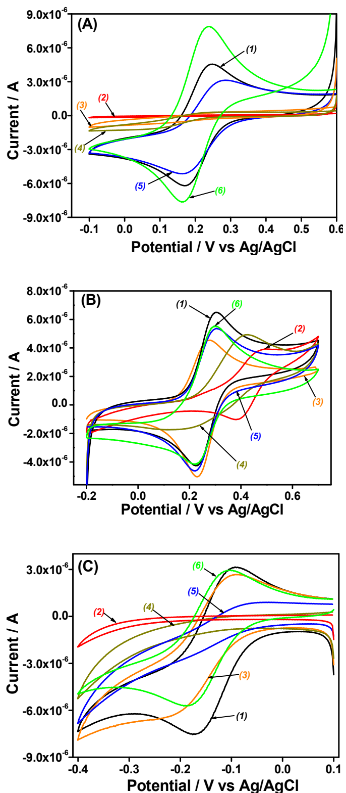
Fig. 4. Cyclic voltammograms recorded in 0.1 M \text{NaNO}_3 containing (A) 0.5 mM [\text{Fe}(\text{CN})_6]^{3-} , (B) 0.5 mM \text{Fc}(\text{MeOH})_2 and (C) 0.5 mM [\text{Ru}(\text{NH}_3)_6]^{3+} , using various electrodes: (1) bare GCE; (2,3) GCE/APTES-Silica before (2) and after surfactant removal (3); (4,5) GCE/APTES-Amino-AT-Silica before (4) and after surfactant removal (5); (6) GCE/Amino-AT. The potential scan rate was 50 \text{ mV s}^{-1} in all cases.
