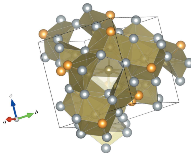
Figure 2 The anion-centred description of the crystal structure of petzite. In this description, tellurium is almost at the centre of a triangular face of a monocapped flattened trigonal antiprism \text{Te}[\text{Ag}_6\text{Au}] . Figure drawn with VESTA.
