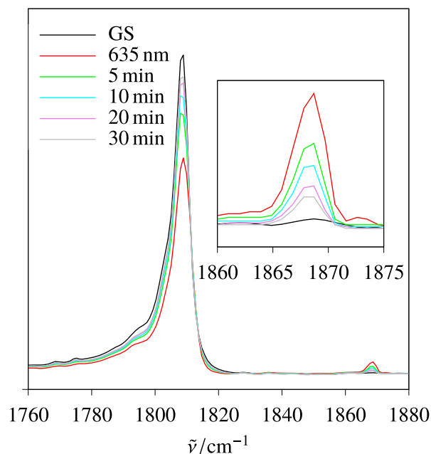
Figure 17. Population at 635 nm and subsequent relaxation of small amounts of a tentative one-electron transfer couple \text{PPN}^+ + [\text{FeCl}_3(\text{NO})]^- in solid \text{PPN}^+[\text{FeCl}_3(\text{NO})]^- . Note the decrease and the re-constitution of the major ground-state N–O stretch, and the population and relaxation of the excited state at 1868\text{ cm}^{-1} .
