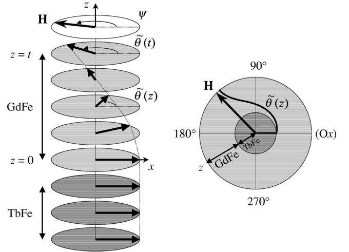
FIG. 3. (Left) Schematic representation of the spin structure forming in the TbFe/GdFe bilayer as the external field \mathbf{H} is rotated counterclockwise an angle \psi away from the easy axis direction Ox . (Right) Polar plot of the corresponding depth dependence of the magnetization angle \tilde{\theta}(z) .
