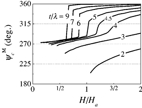
FIG. 7. Calculated evolution of the critical angle of chirality reversal \psi_c^M as a function of the reduced field H/H_a , for various normalized thicknesses t/\lambda of the soft layer.
