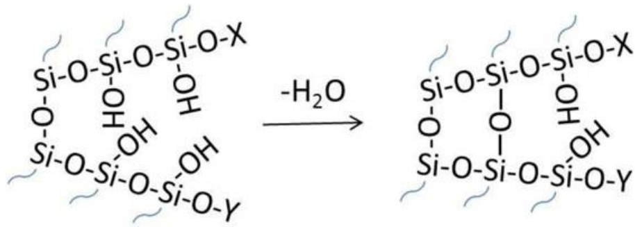
Figure 12: Illustration of a crosslinking reaction between two OH groups in an oligomeric group leading to the loss \Delta m = 18 and the removal of a \text{H}_2\text{O} molecule
