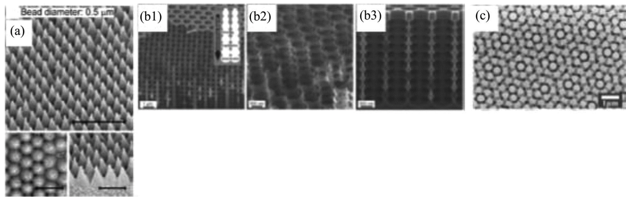
FIGURE 12: (a) SEM images of Teflon nanocone arrays fabricated with 0.5 μm PS beads. The top row shows large tilted views. In the bottom row, left and right images show top view and side view of nanocones, respectively. The scale bars indicate 2 and 1 μm, respectively. Reprinted with permission of ACS.[94] (b) SPRIE designs. (b1 and b2) Hexagonal, (b3) lattices obtained using different colloidal nanosphere arrangements. Reprinted with permission of Wiley.[100] (c) Nanopattern of a bilayer crystal after RIE. Reprinted with permission of ACS.[101]
