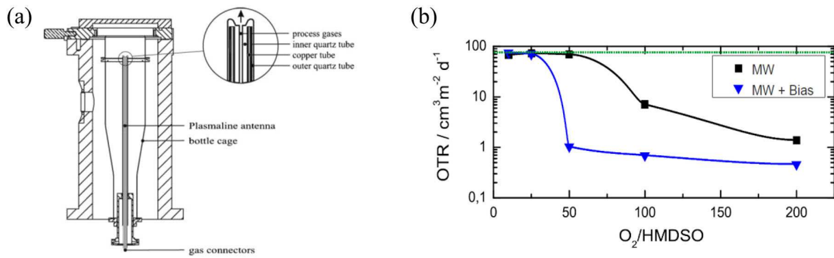
FIGURE 6: (a) Schematic of the reactor system for gas barrier layer deposition on the inner surface of a PET bottle. Height and diameter of vacuum vessel are 400 and 140 mm, respectively. Diameter of bottle cage is 85 mm, and diameter of the microwave Plasmaline antenna (inset) is 12 mm. Reprinted from Deilmann et al. , [39a] with permission from Wiley. (b) OTR of coated PET foils as function of O 2 /HMDSO ratio with a substrate bias of 36 V (MW + bias) and grounded substrate holder (MW). PET foil OTR reference is indicated as dashed line. Image extracted from Mitschker et al. [39c]
