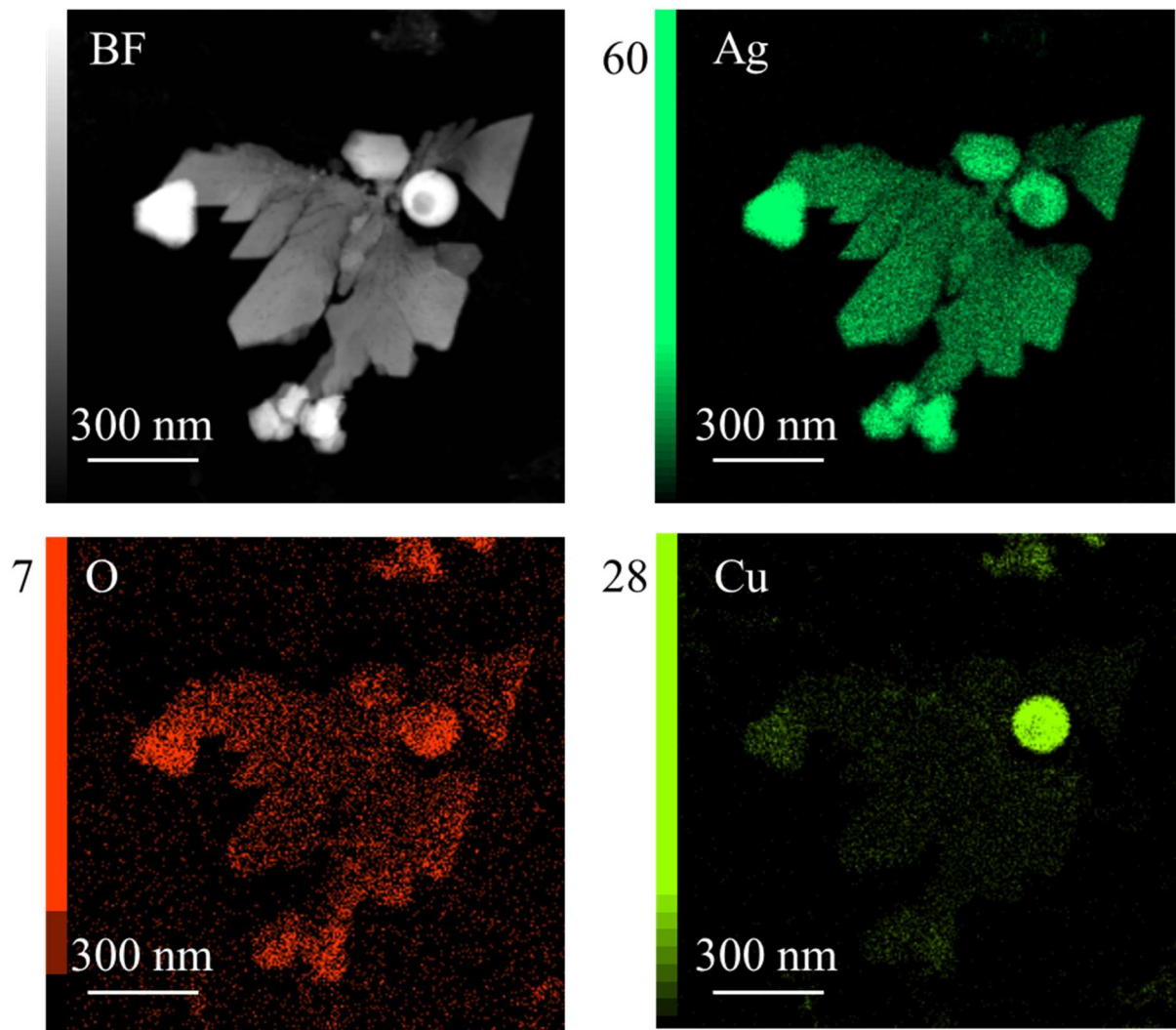
Figure 7: X-mapping of two-dimensional objects shown in the Bright Field image. Ag, O and Cu maps are depicted together with their intensity colour scales whose maximum values are indicated by the given numbers.
