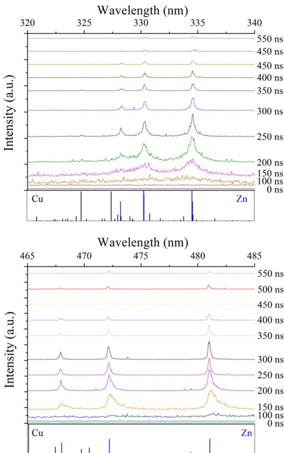
Supplemental Material 3: Time-resolved optical emission spectra recorded for selected wavelength ranges. +10 kV discharges between one Cu electrode (HV) and one zinc electrode (grounded). Spectra were recorded with a 1200 grooves \text{mm}^{-1} grating.
