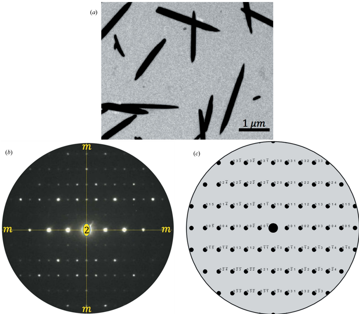
Figure 4 (a) Nanosheets oriented edge on in TEM with the corresponding (b) experimental and (c) simulated electron microdiffraction patterns recorded along the [100] = [2\bar{1}\bar{1}0] zone axis. The experimental pattern shows a (2mm) ideal symmetry for the ZOLZ pattern.
