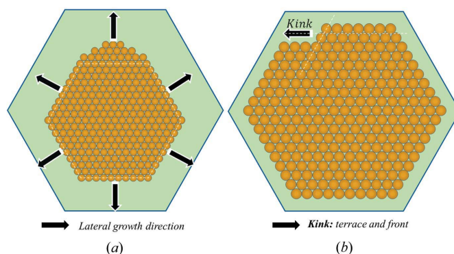
Figure 8 (a) Schematic representation of the radial growth of the lead nanosheet. At the mesoscopic level, the nanosheets are convex and can be decorated by kinks (Fig. 7). On one of the prism faces in (a), the convexity is exaggerated to emphasize the radial expansion of the nanosheet. (b) Presence of a kink on one lateral face.
