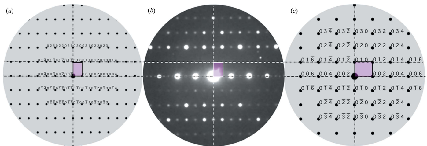
Figure 5 Comparison of the (b) experimental electron diffraction pattern with the (a), (c) simulated ones for the four space groups (a) P6/m2/m2/m and (c) P6/m2/c2/c , P6_3/m2/m2/c and P6_3/m2/c2/m . All the simulated patterns are recorded along the [100] = [2\bar{1}\bar{1}0] zone axis. Only the diffraction pattern of (a) the P6/m2/m2/m space group matches with (b) the experimental one.
