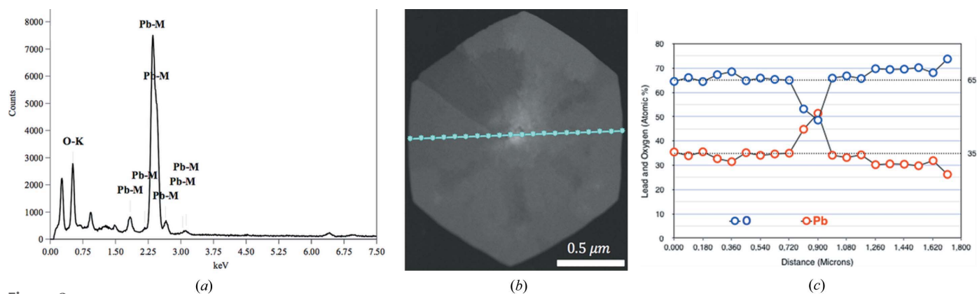
Figure 2 (a) A TEM-EDS spectrum revealing the presence of lead and oxygen elements in a nanosheet. (c) Radial profile of lead and oxygen along the dotted line in (b), recorded by energy dispersive spectroscopy (TEM-EDS) in STEM mode on a lead dioxide particle with hexagonal shape. The bright contrast of the HAADF-STEM image (b), sensitive to the high atomic number, indicates a higher concentration of lead in the central zone ( \text{PbO} ) than in its surroundings ( \text{PbO}_2 ).
