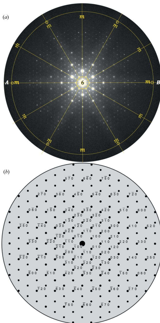
Figure 3 (a) Experimental and (b) the corresponding simulated (ZOLZ) electron microdiffraction patterns recorded along the [001] = [0001] zone axis, showing \{6mm, 6mm\} ideal symmetry for the whole pattern WP = (ZOLZ + FOLZ). The small circles in (a) mark the reflections belonging to the FOLZ indicated by the great circle. The radius of the circle is denoted by R_{FOLZ} .
