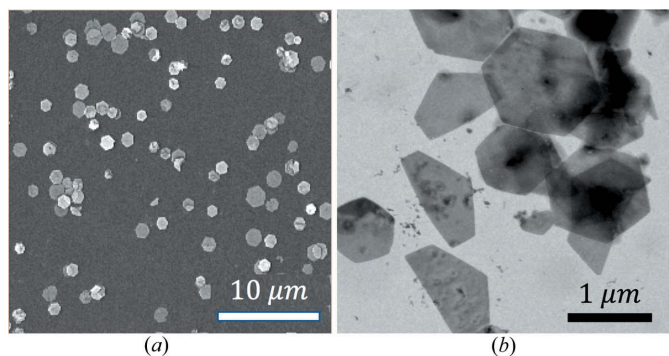
Figure 1 (a) Scanning electron microscopy and (b) bright-field TEM images showing lead dioxide particles with hexagonal shape, deposited on silicon (a) and TEM carbon grid (b) substrates.
