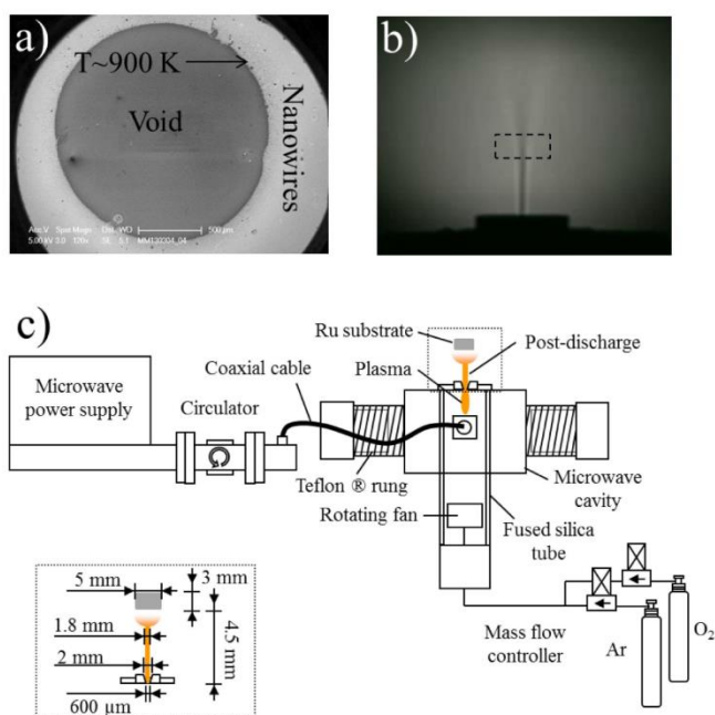
Fig. 1. a) Transition at 900 K between the void and the nanowire outer ring (in this example, a silicon wafer coated by a 1 μm-thick \text{RuO}_2 PVD coating is used as sample). b) Shadowgraphy image of the afterglow beam. The position of the ruthenium substrate is depicted by the dotted line. c) The experimental set-up.
