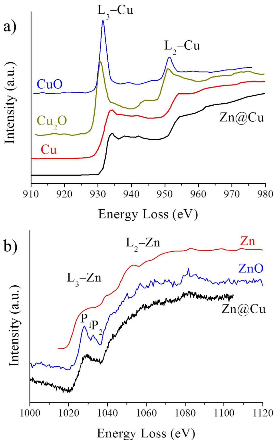
Figure 5: Starting with zinc electrodes. a) Electron Energy Loss Spectroscopy near-edge fine structures for the Cu L 2,3 . b) Electron Energy Loss Spectroscopy near-edge fine structures for the Zn L 2,3 . Reference spectra for CuO, Cu 2 O, Cu are taken in [19] whereas reference spectra for Zn and ZnO are taken in [20] and [21] respectively.
