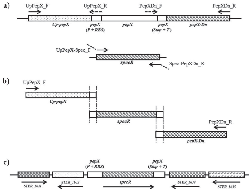
Figure 1. Schematic representation of different steps of overlap extension PCR to replace the pepX gene by the specR gene and resultant mutant locus. (a) Amplification of the PepX upper flanked region (UpPepX), resistance to antibiotic spectinomycin ( specR ), and PepX down flanked region (PepXDn) fragments using appropriate primer pairs. (b) The overlap extension PCR using the outermost primer pair and the 3 amplicons. (c) The resulting chromosomal locus carrying the specR gene obtained after transformation with the final overlap extension PCR amplicon. Dotted lines indicate the homologous/complementary regions. P, RBS, stop, and T correspond to promoter, ribosome binding site, stop codon, and transcription terminator of pepX gene, respectively.
