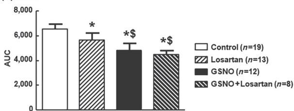
FIGURE 3 S-nitrosoglutathione (GSNO) decreases AT 1 receptor-dependant myogenic tone. Impact of an exposure to GSNO (2 × 10 -6 mol·L -1 , 30 min followed by a 1-hr washout), losartan (10 -5 mol·L -1 ), or the combination GSNO + losartan on (a) myogenic tone and (b) AUC of myogenic tone of middle cerebral arteries isolated from Wistar rats. Values are expressed as means ± SEM. One-way ANOVA (treatment) was used to calculate P values; * P < 0.05 versus control; § P < 0.05 versus losartan; * P < 0.05 versus control (Bonferroni post-test)
