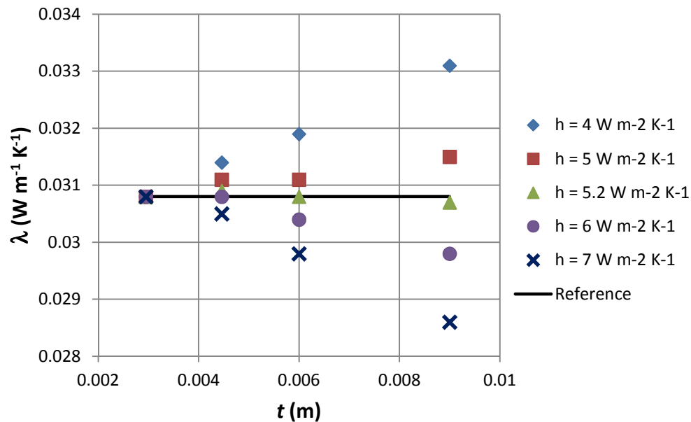
Figure 5. Estimated thermal conductivity of the XPS foam samples, \lambda , using various values of the exchange coefficient, h .
