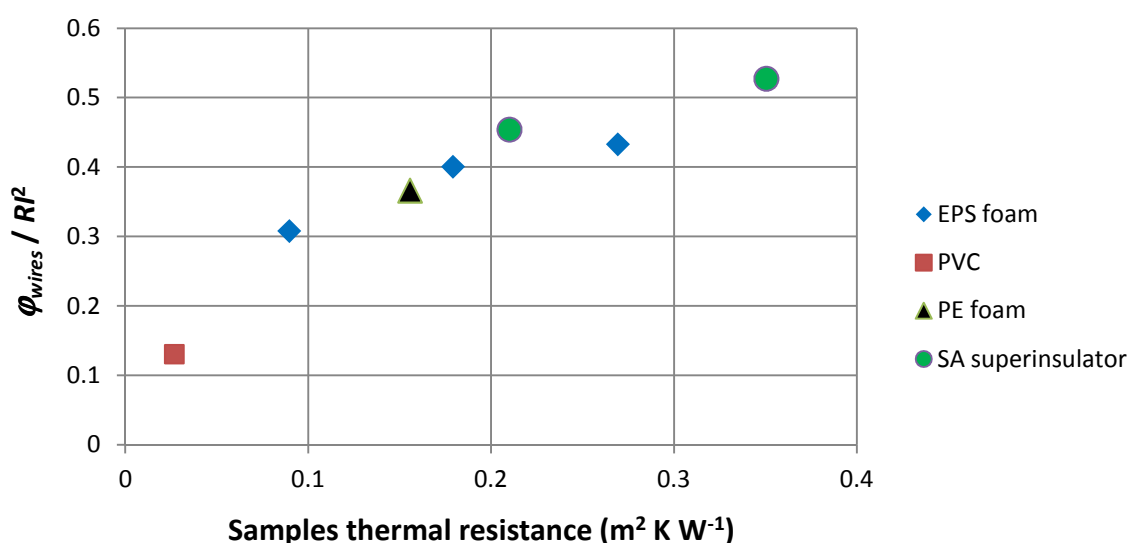
Figure 6. Ratio of the heat flow rate lost through the wires to the conduction heat flow rate, \phi_{wires} / R\dot{I}^2 , as a function of the samples thermal resistance.
