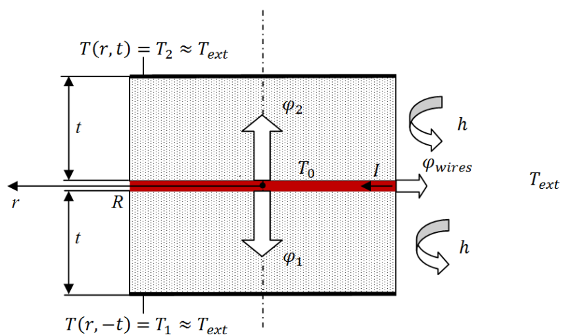
Figure 2. Schematization of the heat flows in the CTHP method
