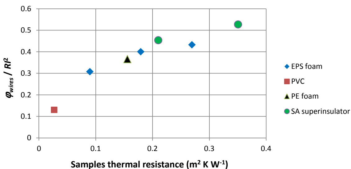
Figure 6. Ratio of the heat flow rate lost through the wires to the conduction heat flow rate, \phi_{wires} / RI^2 , as a function of the samples thermal resistance.
