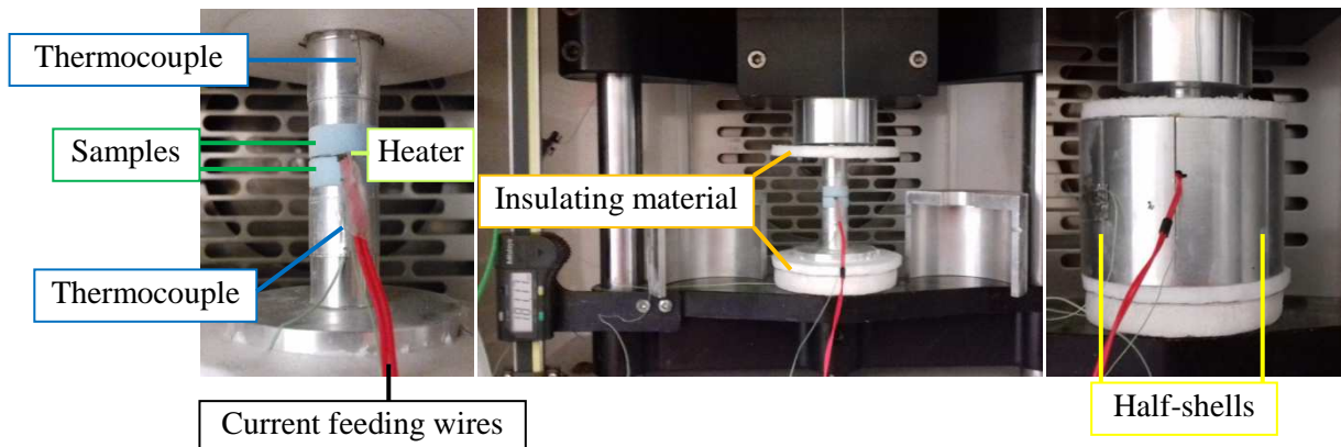
Figure 4. Side views of the lab-made device. From left to right: detail of the heater sandwiched between two identical samples (here XPS foam), themselves inserted between 2 aluminum blocks; general view of the setup gently compressed for allowing good thermal contacts; setup closed with half shells in the climate chamber.
