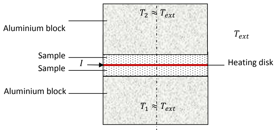
Figure 1. Block diagram of the experimental setup
