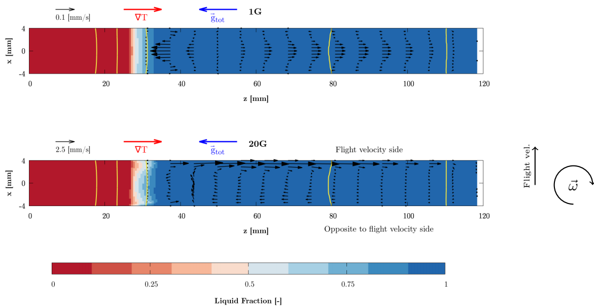
Figure 5. Comparison of the liquid convection between the 1G and 20G cases at t = 300[s] . Temperature contours in yellow from left to right: 1400,1450,1500,1550 [ ^{\circ}C ].
