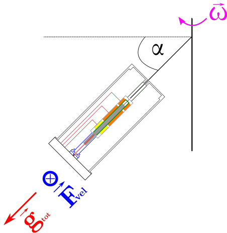
Figure 3. Schematic of the furnace and the sample in the centrifuge. Ti-Al sample (grey), heaters (yellow and orange) and thermocouples (red).
