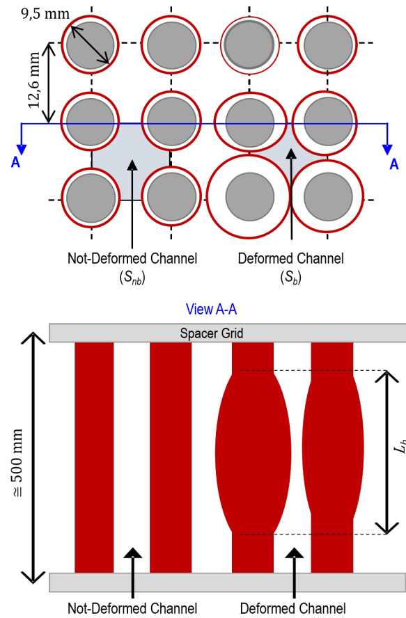
Figure 4: Illustrative drawing of a sub-channel representation.
