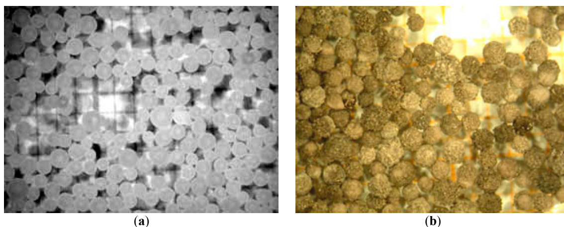
Figure 11. VM views of sodium hydroxide at: (a) Initial state, \leq 1 \text{ mm} ; (b) After reacting with powder iron sulfate.
