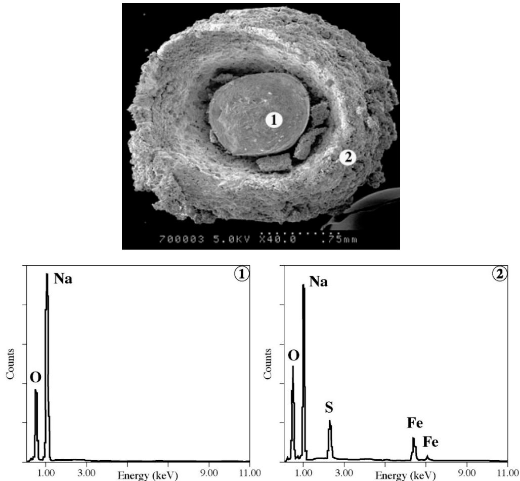
Figure 6. Scanning electron microscope coupled with energy dispersive spectrometry (SEM-EDS) examination results of a NaOH pellet reacted with \text{FeSO}_4 \cdot \text{H}_2\text{O} : (1) core of the NaOH pellet; (2) outer part of the NaOH pellet.
