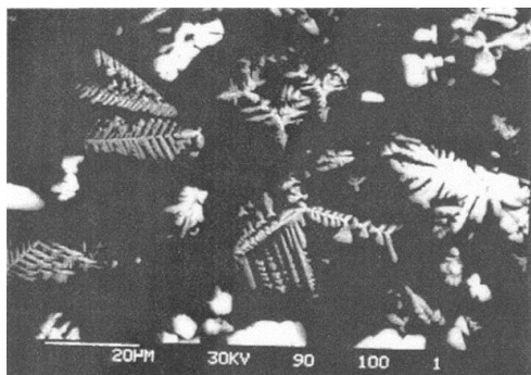
Figure 10. SEM/EDS aspects of the tin slag before (a) and after leaching (b).
