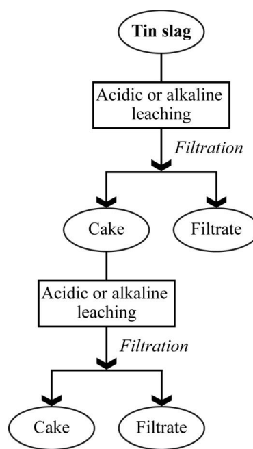
Figure 4. Experimental procedure for the leaching of tin slags.
