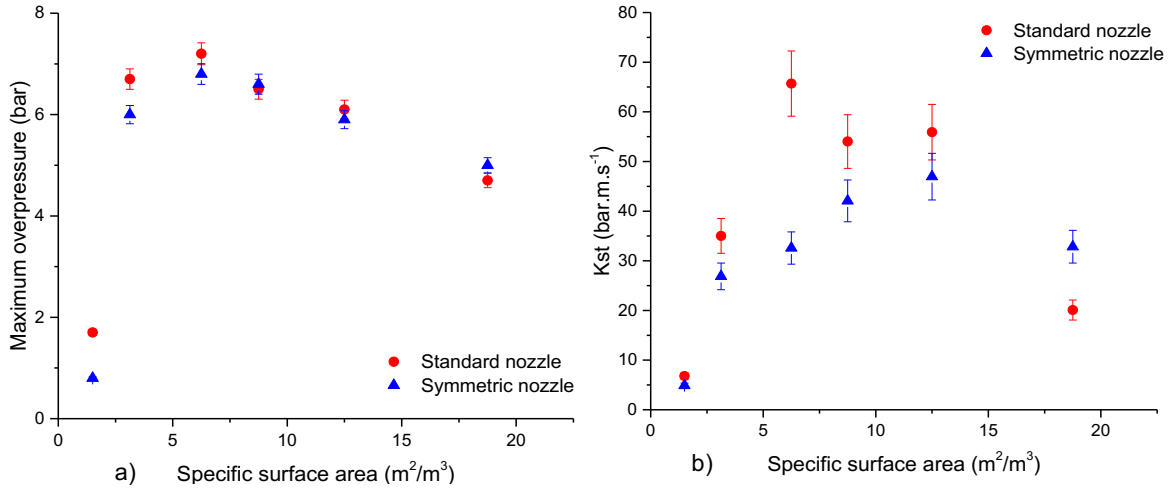
Figure 1: (a-left) Maximum overpressure and (b-right) dust deflagration index K_{St} of carbon black nanoparticles with two different nozzles as a function of the total surface area of particles per cubic meter of cloud
