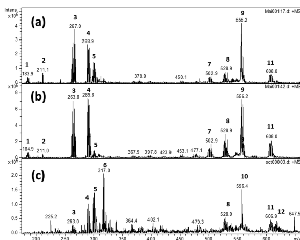
Fig. 9 ESI-MS spectra of (a) \Phi_{\text{S,1}} , (b) \Phi_{\text{S,2}} and (c) \text{Pd}(\text{CN})_2 after partial dissolution in pyridine (solid : liquid ratio = 2 \text{ g L}^{-1} ) and dilution in acetonitrile ((a) 1/10^{\text{th}} , (b) 1/100^{\text{th}} and (c) 1/10^{\text{th}} ). Experiment conditions: trap drive setting = 50; skimmer voltage = 30 V.
