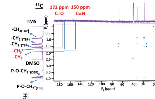
Fig. 12 2D NMR spectrum of ^1\text{H} and ^{13}\text{C} (pulse sequence gHMBCAD) of \Phi_{s,2} partially dissolved in DMSO-D6 with m(\Phi_{s,2}) = 9.8 mg in 650 \mu\text{L} of DMSO-D6 ( S/L = 15.07 g of precipitate/L of solvent).
