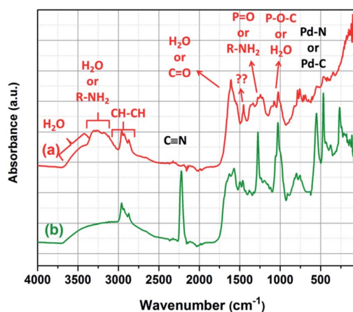
Fig. 7 IR spectra of (a) \Phi_{\text{S},3} (solid residue after dissolution of the \Phi_{\text{S},1} in 1 \text{ mol L}^{-1} \text{ NH}_3 ) and (b) \Phi_{\text{S},1} .
