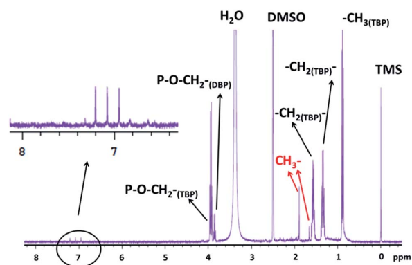
Fig. 10 1D ^1\text{H} NMR spectrum of \Phi_{S,2} partially dissolved in DMSO- \text{D}_6 m(\Phi_{S,2}) = 9.8 mg in 650 \mu\text{L} of DMSO- \text{D}_6 , i.e. S/L = 15.07 g of precipitate/L of solvent.
