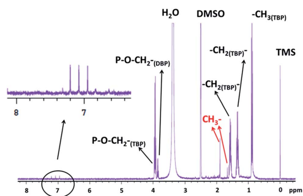
Fig. 10 1D ^1\text{H} NMR spectrum of \Phi_{\text{S},2} partially dissolved in DMSO- \text{D}_6 m(\Phi_{\text{S},2}) = 9.8 mg in 650 \mu\text{L} of DMSO- \text{D}_6 , i.e. S/L = 15.07 g of precipitate/L of solvent.
