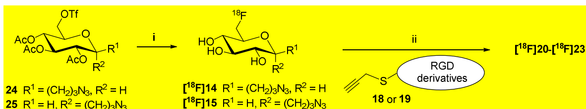
Scheme 4. Radiosynthesis of [\text{18F}]\text{F} -C-glyco"RGD" derivatives [\text{18F}]\text{20} - [\text{18F}]\text{23} . Reagents and conditions: (i) 1) \text{K}[\text{18F}]\text{F-K}_{222} , \text{CH}_3\text{CN} , 95^\circ\text{C} , 5 min, decay-corrected radiochemical yields (48 to 69%). 2) HPLC purification. 3) \text{NaOH} , 30^\circ\text{C} , 9 min then \text{HCl} . (ii) \text{Cu}(\text{OAc})_2 , Na ascorbate, \text{H}_2\text{O} , 55^\circ\text{C} , 25 min, (40 to 65 %).
