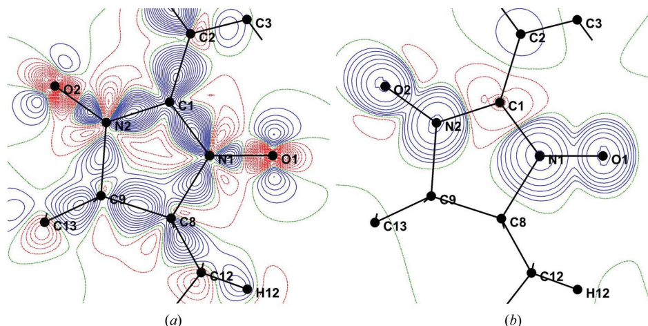
Figure 3 Experimental static deformation electron density ( a , contour intervals of 0.05 \text{ e } \text{Å}^{-3} ) and spin density ( b , contour intervals of 0.01 \times 2^n \mu_B \text{ Å}^{-3} ) in the plane of two NO groups [positive (blue) negative (red) and neutral (green)].
