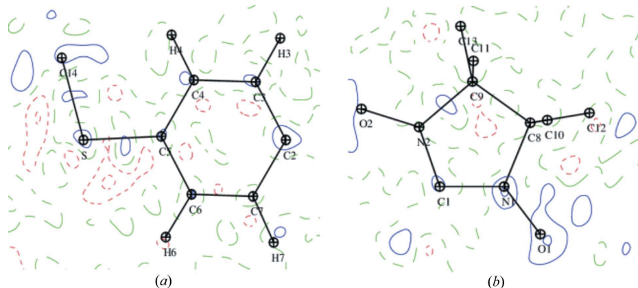
Figure 2 Residual electron density maps in the phenyl ring plane ( a ) and Nit ring ( b ) plane. Contour intervals of 0.05 \text{ e } \text{Å}^{-3} , positive (blue), negative (red) and neutral (green) lines.
