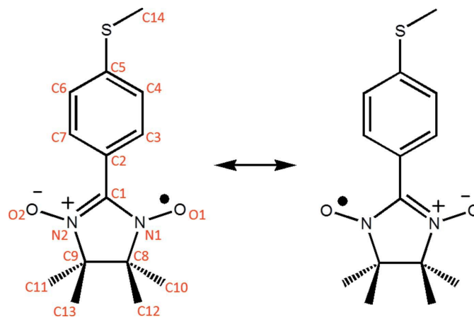
Figure 1 Main resonance structures of Nit(SMe)Ph. On the left one, the labels of the main atoms are reported, while H atoms are omitted for the sake of clarity.
