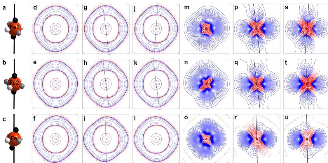
Figure 2 | Electron density distributions in 1 and 2. a-c , Locations of the Laplacian minima (charge concentrations) determined for the iron atoms in 1 ( a,b ) and 2 ( c ) marked as white, gray, and black spheres. d-l , Laplacian contour maps with a width of 1 \text{ \AA} for iron atoms in 1 and 2 . m-u , Static model deformation electron density maps with a width of 2.2 \text{ \AA} for iron atoms in 1 and 2 . The planes in these maps are defined from the positions of the minima in a-c . The maps in the first column ( d-f , m-o ) include white and gray spheres, the maps in the second column ( g-i , p-r ) include the black and white spheres, and the maps in the third column ( j-l , s-u ) include the black and gray spheres. Solid blue lines represent positive contours of -\nabla^2\rho (local charge concentration) and the static model deformation electron density. Dashed red lines represent negative contours of -\nabla^2\rho (local charge depletion) and the static model deformation electron density. Laplacian contours are drawn at \pm 2, 4, 8 \times 10^n \text{ e}/\text{\AA}^5 , where n is an integer ranging from -3 to +3 . An additional contour is drawn at -\nabla^2\rho = 1000 \text{ e}/\text{\AA}^5 to emphasize the different
