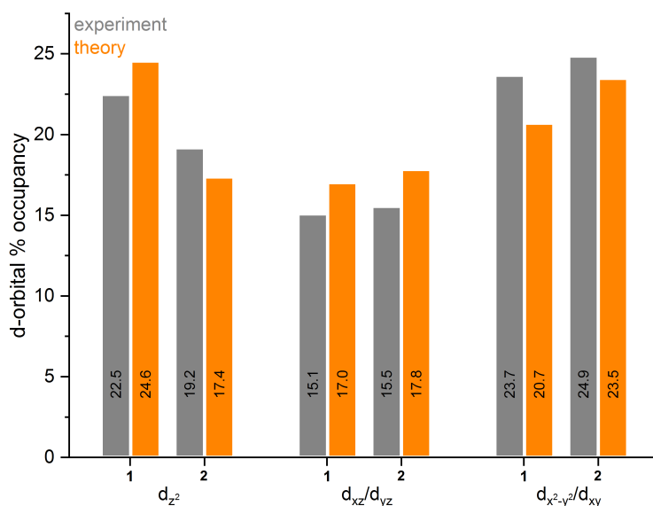
Figure 3 d-orbital occupancies from experiment and theory. Occupancies derived from multipole population parameters using experimental (grey) and theoretical (orange) structure factors. Occupancy averages (as percentages of the valence electron count) are reported for the nearly degenerate ( d_{xz} , d_{yz} ) and ( d_{x^2-y^2} , d_{xy} ) pairs of orbitals.
