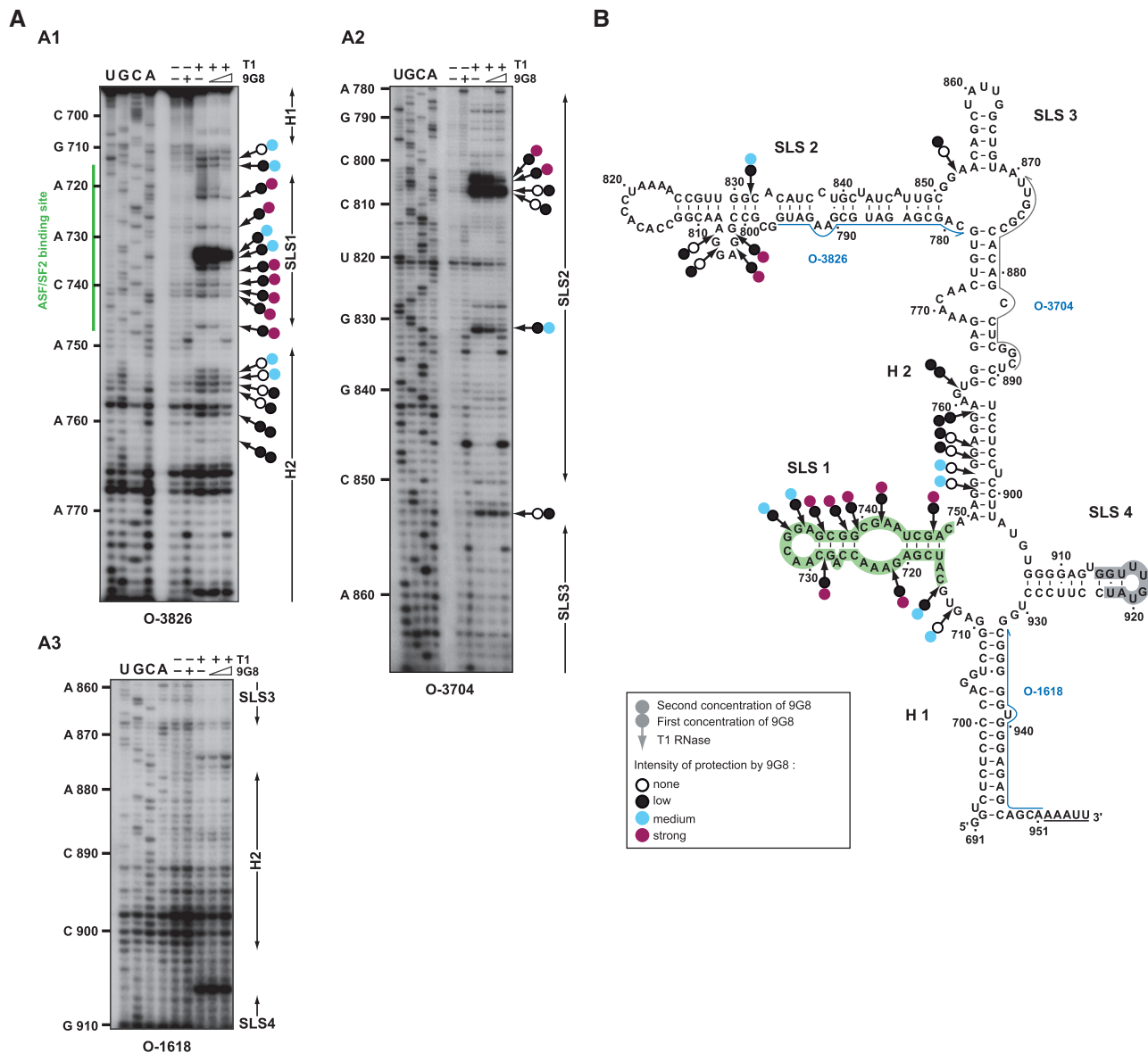
Figure 7. Enzymatic footprinting of 9G8 binding sites on RSV NRS RNA. (A1–A3) Primer extension analyses of RSV NRS cleaved by T1 RNase in the absence or the presence of protein 9G8. RNA-protein complexes were formed at [9G8]/[RNA] molar ratios of 25 and 50, respectively. The absence of protein addition is indicated by (–). Enzymatic reactions were performed as described in ‘Materials and Methods’ section. Lanes U, G, C and A correspond to the sequencing ladder and primers used for reverse transcription are indicated below each autoradiogram. Nucleotide numbering in the RSV NRS RNA and positions of the ASF/SF2 (19) binding site are indicated on the left side of the autoradiogram. Positions of helices (H) and stem–loop structures (SLS) are shown on the right side of the autoradiograms. Cleavages by T1 RNase and protection generated by protein 9G8 are represented by arrows with two circles. Colours of the first and second circles represent the level of protection obtained at the 25 and 50 [protein]/[RNA] molar ratios, respectively (white, black, blue and purple for none, low, medium and strong protection, respectively). (B) Schematic representation of the protections generated by protein 9G8 is depicted on the RSV NRS RNA 2D structure using the same rules as in A. Primers are indicated by blue arrows. The ASF/SF2 and snRNA U1 binding sites according to references (17,19) are highlighted in green and grey, respectively.
