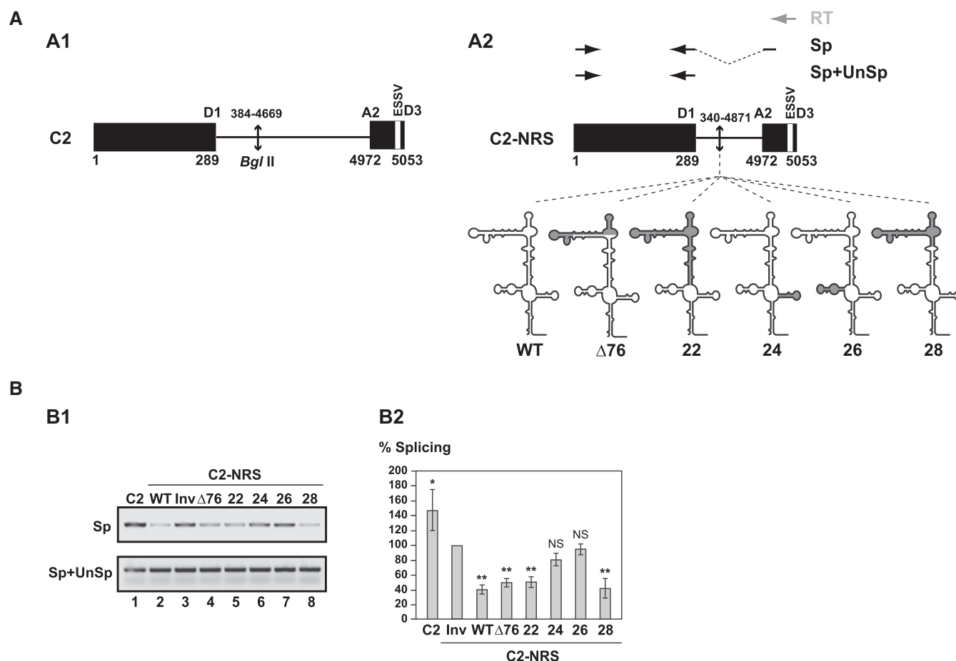
Figure 3. Comparison of splicing inhibition properties of NRS WT and \Delta 76 , 22, 24, 26 and 28 NRS variants in the C2 pre-mRNA context. (A) Schematic representation of the HIV C2 pre-mRNA (A1) (31) and C2-NRS heterologous pre-mRNAs (A2). Black boxes and thin lines represent exons and intron, respectively. Numbering of C2 RNA is according to (49). End-joining of the two HIV-1 sequences in the C2 intron is depicted by an arrow. The D1 5'-ss and A2 HIV-1 3'-ss as well as the ESSV regulatory element are shown (43). Heterologous C2-NRS constructs, created by insertion of the WT and variant \Delta 76 , 22, 24, 26 and 28 NRSs in the intron, are schematically represented below. Segments deleted in the variant NRS elements are in grey. The RT (in grey), and PCR (in black) primers used for evaluation of the yields of C2 and C2-NRS pre-mRNAs splicing efficiencies are represented by arrows above the C2-NRS construct. Yields of spliced RNAs (Sp) and of spliced plus unspliced products (Sp+UnSp) were analysed by PCR amplifications using the pairs of primers marked by Sp and Sp+UnSp, respectively. (B) RT-PCR analysis of in vitro splicing products of the C2 and heterologous C2-NRS pre-mRNAs. In vitro splicing assays were performed as described in 'Materials and Methods' section. Experiments were repeated three times using different batches of RNA (Supplementary Figure S5A). The relative splicing efficiencies of the various constructs were estimated by semi-quantitative RT-PCR performed in triplicate (Supplementary Figure S5A). A representative example of cDNA fractionation obtained for each of the tested pre-mRNAs is shown (B1). Identities of RT-PCR products spliced (Sp) or spliced plus unspliced (Sp+UnSp) products are indicated. The identity of the pre-mRNA used in the assay is given above the lane. The Sp/Sp+UnSp pre-mRNA ratio obtained for the C2-NRS Inv construct was taken as the reference (100%). The Sp/Sp+UnSp ratios established for the other constructs are given as a percentage of this reference. The mean values of the Sp/Sp+UnSp percentages determined for three independent splicing reaction and their standard deviations are given (B2). * P < 0.05 , ** P < 0.01 , NS: not significant.
