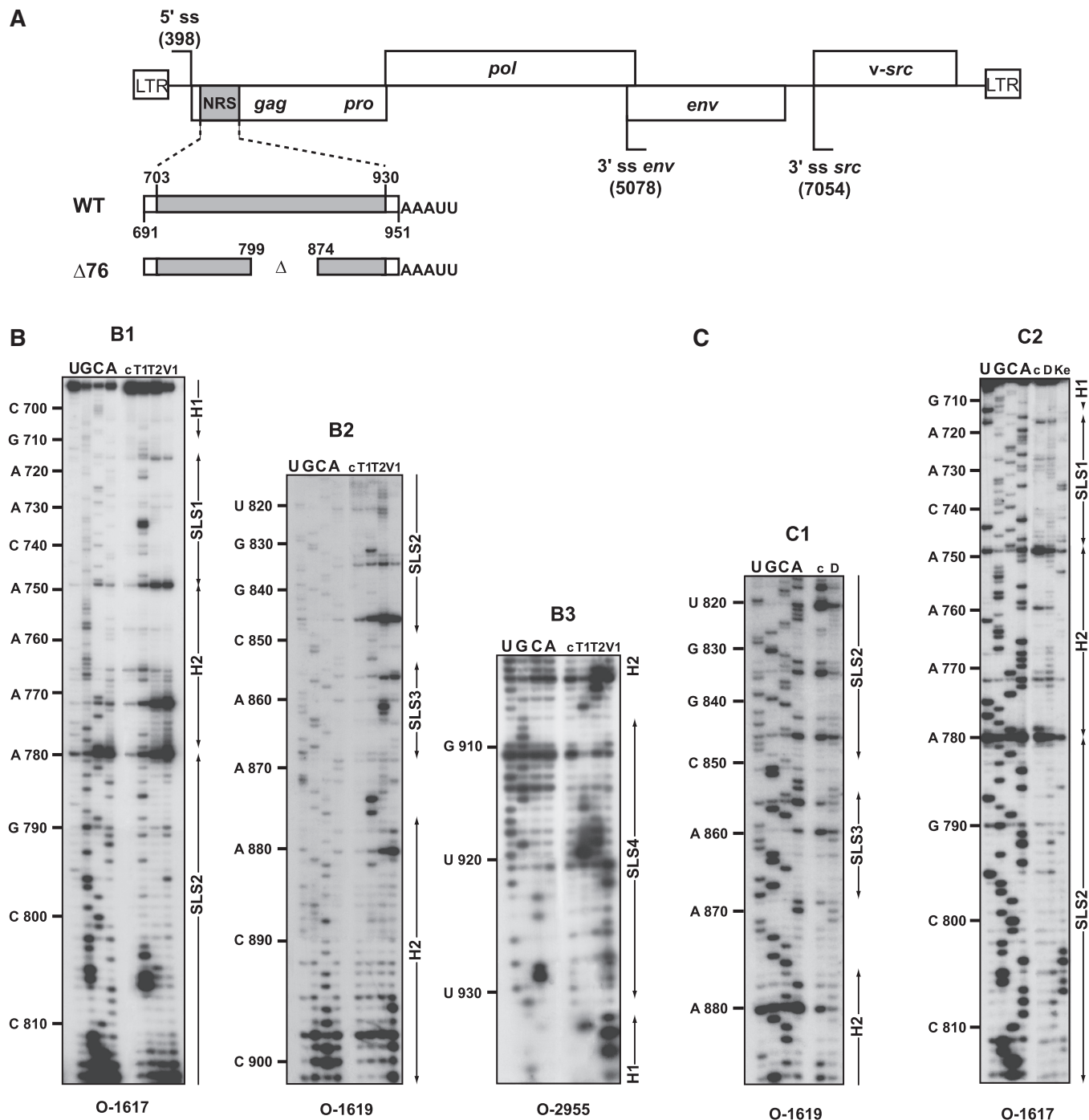
Figure 1. (A) Schematic representation of the RSV Prague C (PrC) genome and of the NRS RNAs used for secondary structure analyses. The architecture of the RSV PrC genome is shown on top of the Figure. The 5'-ss and 3'-ss are indicated and boxes represent the open reading frames. The grey box depicts the NRS element (nucleotides 703–930) located in the gag gene used for secondary structure experiments. Viral sequences belonging to the RSV segments located upstream and downstream from NRSs are in white. The non-viral AAAUU sequence at the 3'-end of the transcripts is shown. Delimitations of NRS are indicated according to NRS nucleotide numbering (48). (B and C) Primer extension analyses of enzymatic cleavages and chemical modifications of NRS WT. (B) Primer extension analyses of enzymatic cleavages in NRS WT (position 691–951) (B1–B3), (C) primer extension analyses of chemical modifications in NRS WT (position 710 to 890) (C1 and C2). T1, T2, V1, D and Ke above the lanes indicate T1, T2, V1 RNase digestions and DMS or Kethoxal modifications, respectively. Conditions for digestions, modifications and reverse transcription are given in 'Materials and Methods' section. Lanes c correspond to control experiments with untreated RNA; lanes U, G, C and A correspond to the sequencing ladder. Primers used for reverse transcription are indicated below each autoradiogram (see Supplementary Table S1 for their nucleotide sequences). Nucleotide numbering according to (48) is indicated on the left side of the autoradiograms. Positions of the stem-loop structures (SLS1, SLS2, SLS3 and SLS4) and the helices (H1 and H2) are shown on the right side of the autoradiograms.
