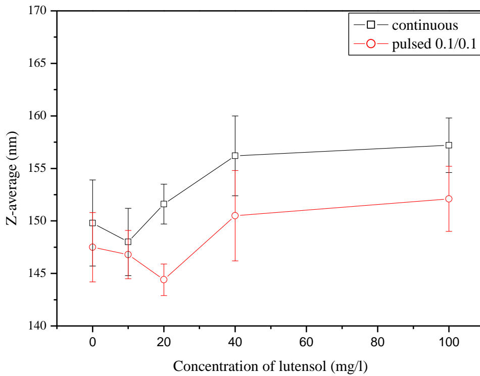
Figure 8: Influence of Lutensol concentration on mean alumina nanoparticle size after 180 s of ultrasonication.
