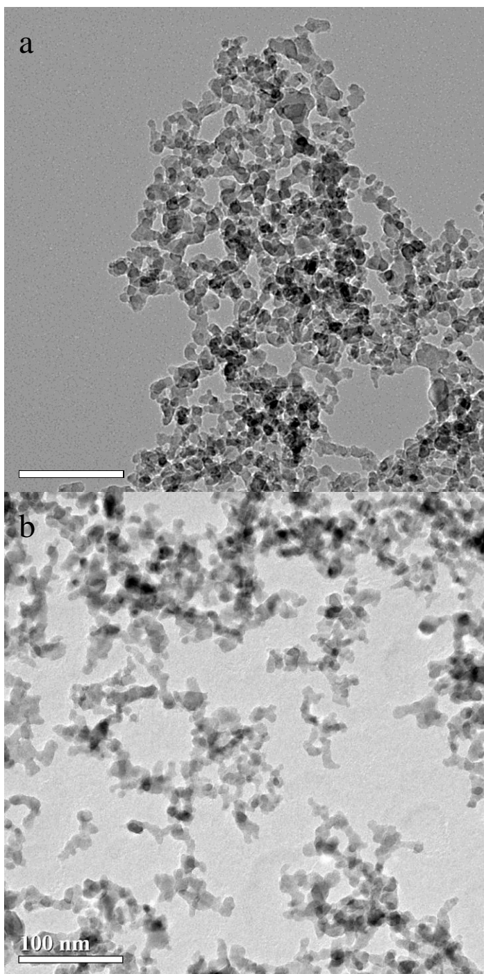
Figure 2 : TEM images of alumina nanoparticles (a) before and (b) after 180 s of ultrasonication at 30 % vibration amplitude.
