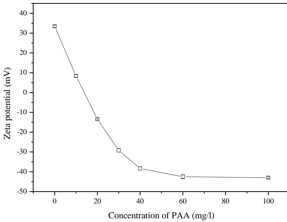
Figure 10 : Influence of PAA concentration on Zeta potential of alumina nanoparticles.
