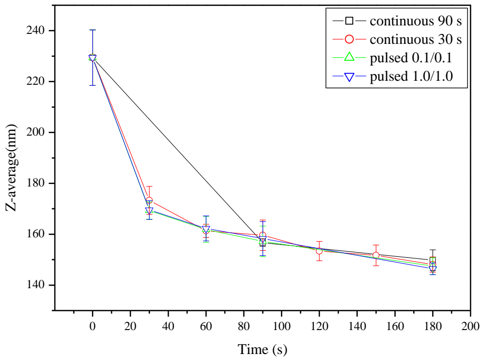
Figure 4 : Influence of ultrasonic modes (continuous and pulsed) on the deagglomeration of alumina nanoparticle at 30 % vibration amplitude.
