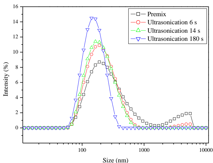
Figure 1: Particles size distribution by intensity of alumina in ultrasonic deagglomeration at 30 % vibration amplitude.
