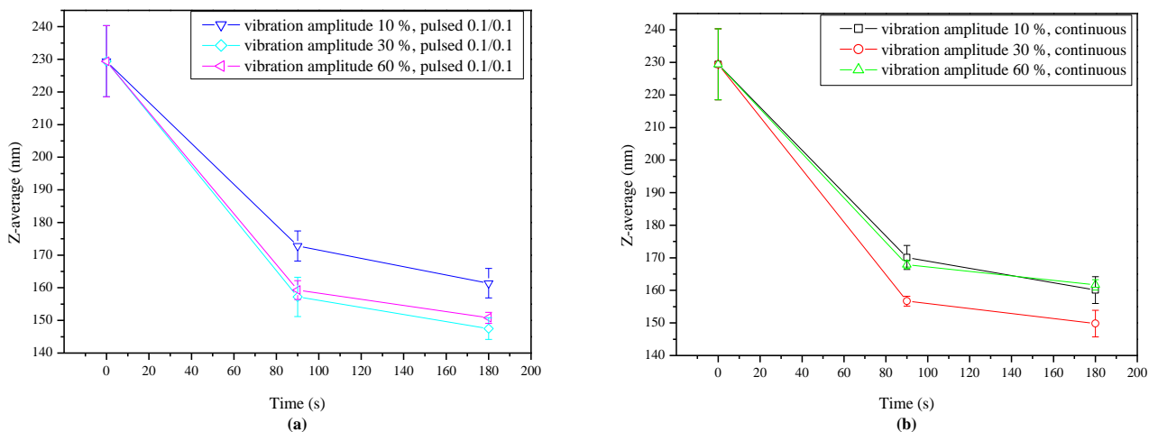
Figure 5 : Influence of vibration amplitude of ultrasound on the deagglomeration of alumina nanoparticles (a) radiation with pulse ratio 0.1/0.1 (s/s) and (b) continuous mode.
