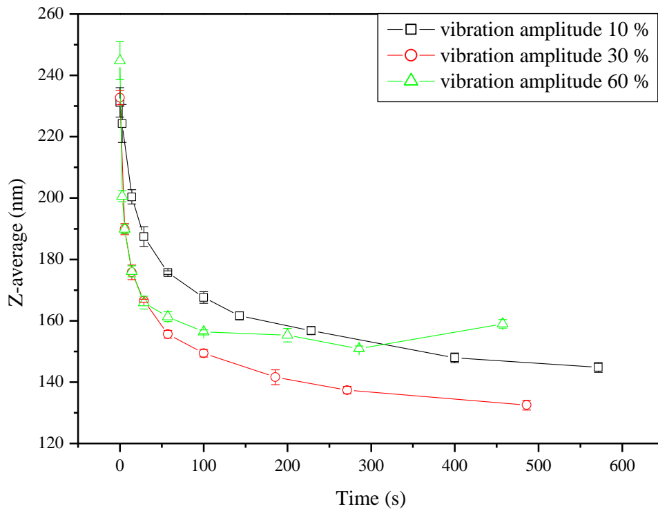
Figure 3: Evolution of mean alumina nanoparticle size at different vibration amplitudes of 10 %, 30 %, 60 % versus ultrasonic time (pulse ratio 0.1/2.0 (s/s)).
