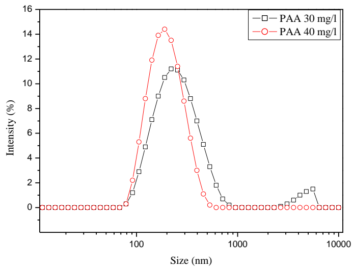
Figure 11: Size distribution by intensity of alumina nanoparticles in suspensions with PAA after 180 s of ultrasonication.
