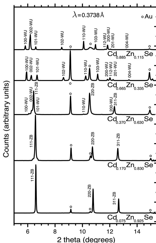
FIG. 2. X-ray \text{Cd}_x\text{Zn}_{1-x}\text{Se} powder diffractograms. Powder X-ray diffraction patterns obtained at (nearly) ambient pressure using the 0.3738 Å radiation (ZB, zincblende; WU, wurtzite). Circles mark diffraction lines due to Au, used for pressure calibration.
