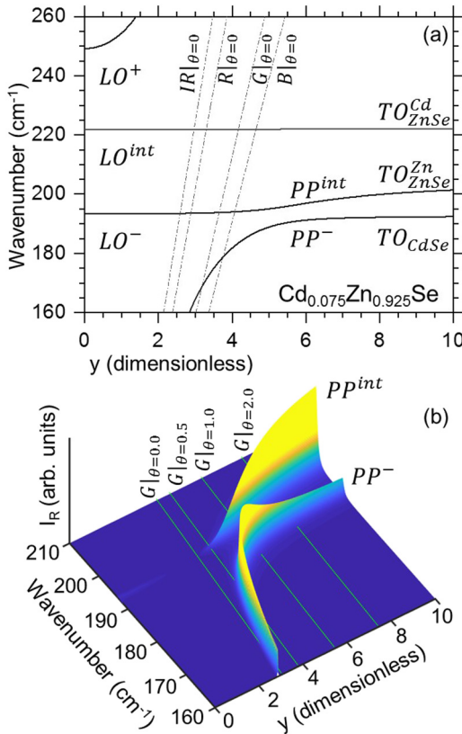
FIG. 8. \text{Cd}_{0.075}\text{Zn}_{0.925}\text{Se-c} PP regime. Theoretical dispersion (a) and the Raman signal (b) of the \text{Cd}_{0.075}\text{Zn}_{0.925}\text{Se-c} PP modes. The Raman scan lines calculated in the perfect forward scattering geometry ( \theta = 0^\circ ) by using the dispersion of the refractive index (Fig. 3) close to the near-infrared (IR, 785.0 nm), red (R, 632.8 nm), green (G, 514.5 nm), and blue (B, 488.0 nm) laser lines (panel a) and in various near-forward scattering geometries ( \theta \sim 0^\circ ) using the green laser line (panel b) are superimposed.
