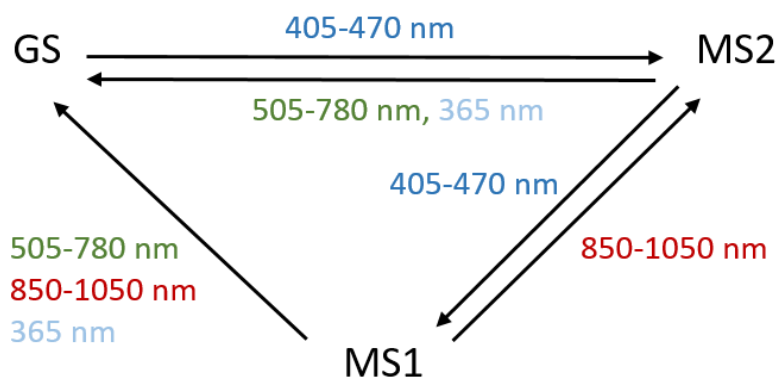
Figure S8. Scheme of linkage isomerization in [\text{RuNO}(\text{Py})_4\text{F}](\text{ClO}_4)_2 indicating relevant spectral ranges for population and depopulation with light.
