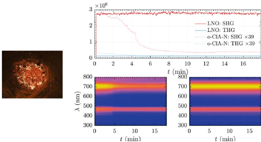
Figure 7. Left: o -CIAN-pellet before exposure. The pellet measures 5 mm in diameter. Right top: second (red) and third (blue) harmonic emission from LNO (solid lines) and o -CIAN (dashed lines) as a function of time. SHG and THG signal of o -CIAN have been scaled for better visibility. Right bottom: normalized spectral traces for o -CIAN (left) and LNO (right) scaling from yellow (high) to blue (low signal).
