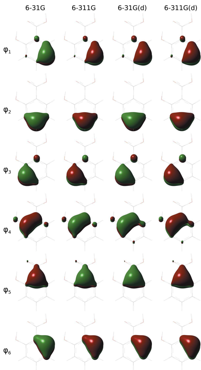
Figure 2 Three-dimensional plots of the unconstrained SC.0 spin-coupled orbitals ( 0.06 e \text{ bohr}^{-3} isosurfaces are plotted). The unconstrained SC.1 spin-coupled orbitals have analogous shapes.
