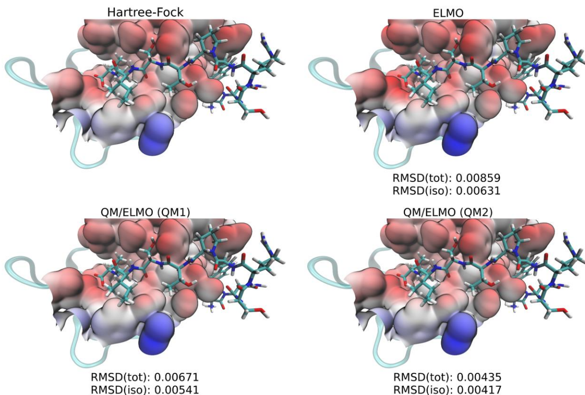
Figure 5. Electrostatic potentials (ESPs) plotted onto the corresponding 0.001 \text{ e/bohr}^3 electron density isosurfaces (BWR color-map in the range [-0.332, 0.035] (values in E_h )). Below the plots of the ELMO and QM/ELMO electrostatic potentials, their RMSD values with respect to the Hartree-Fock ESP are also shown (see section S3.3 of this Supporting Information for more details about the RMSD(tot) and RMSD(iso) indexes).
