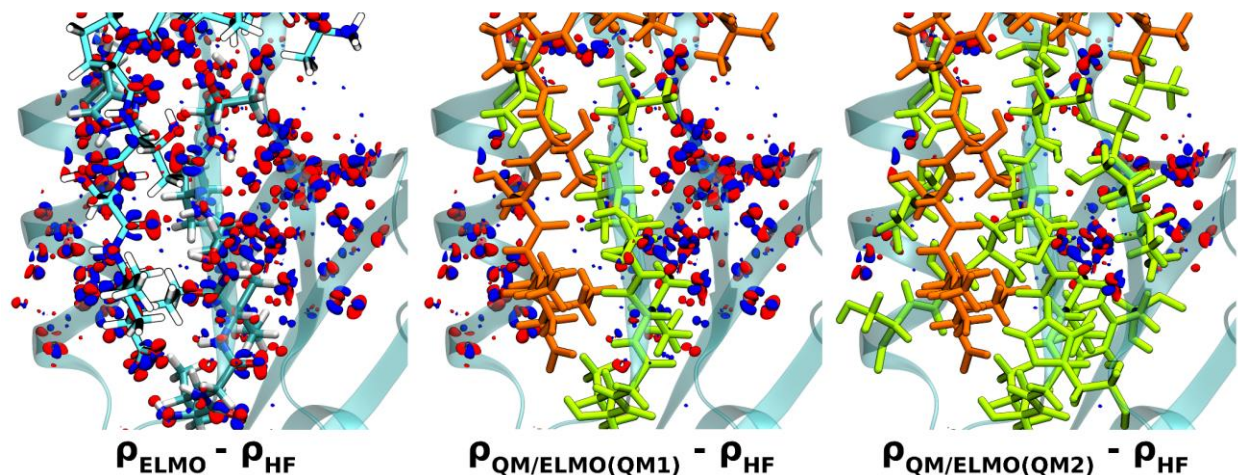
Figure 4. Three-dimensional residual densities obtained comparing the ELMO, QM/ELMO (QM1) and QM/ELMO (QM2) electron distributions to the Hartree-Fock one. The isosurface-values are set to 0.01 \text{ e/bohr}^3 , with positive and negative isosurfaces in blue and red, respectively; in the ELMO case (left panel) the “licorice representation” is only used to highlight the region of the most important intermolecular contacts, while, for the QM/ELMO comparisons (center and right panels), it is used to indicate the QM regions, with the ligand molecule colored in orange and the protein residues in lime green.
