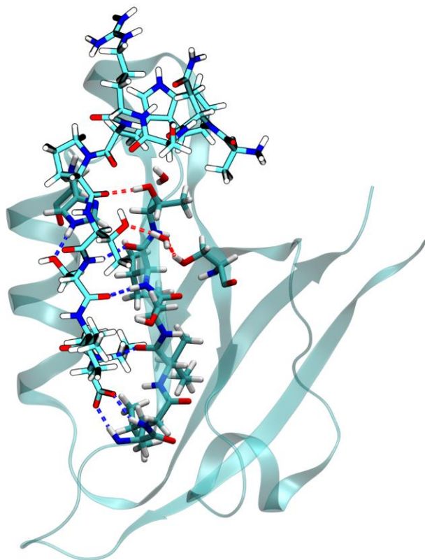
Figure 3. Three-dimensional structure of the protein:ligand complex, with the region of the most important intermolecular contacts in “licorice representation”. Blue dashed lines indicate hydrogen bonds.
