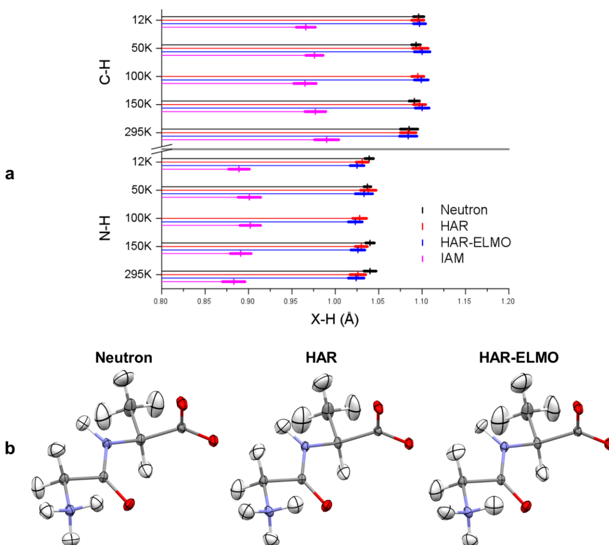
Figure 1. a) Accuracy and precision of bond distances involving hydrogen atoms (X-H) for Gly- L -Ala at all temperatures (note that there is no neutron diffraction experiment at 100 K). Estimated accuracy is expressed by a match of the averaged bond lengths with the reference neutron experiment. Estimated precision is expressed by the size of the error bar, which represents the sample standard deviation upon averaging.
