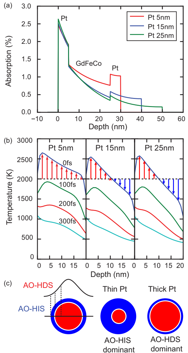
FIG. 5. (a) Calculated light absorption as a function of sample depth for Pt (5 nm)/GdFeCo (20 nm)/Pt ( x nm), x = 5, 15, and 25 . Ta(3) is neglected in the calculation. (b) GdFeCo electron temperature plotted against the depth at 0 (blue), 100 (green), 200 (red), and 300 fs (cyan). 0 fs is defined as the time when the laser pulse stops and the samples are exposed to the laser pulse of 5 \text{ mJ/cm}^2 during -50 to 0 fs. The dashed line indicates the threshold temperature. The magnetization in the hot part (red arrows) tends to switch while the magnetization tends to stay in the original direction in the cold part (blue arrows). (c) The influence of Pt capping: in the case of thin Pt capping, AO-HIS (the outer ring) is dominant; in the case of thick Pt capping, AO-HDS (the inner ring) is dominant.
