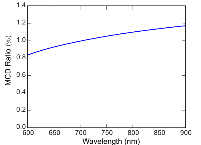
FIG. 7. MCD ratio deduced from ellipsometry measurement is shown as a function of wavelength.
