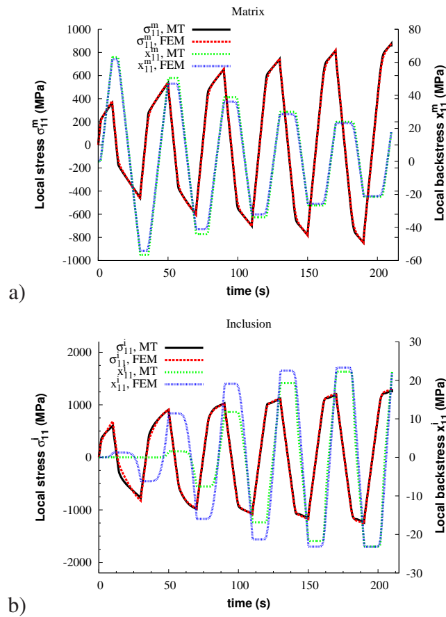
Fig. 9. Time evolution during cycles of the mean longitudinal stress (left axis) and backstress (right axis) in the a) matrix domain, b) inclusion phase. The two phases are elastic-viscoplastic with combined isotropic and linear kinematic hardening. The volume fraction of inclusions is c = 0.25 . The material parameters are those of Fig. 8.
