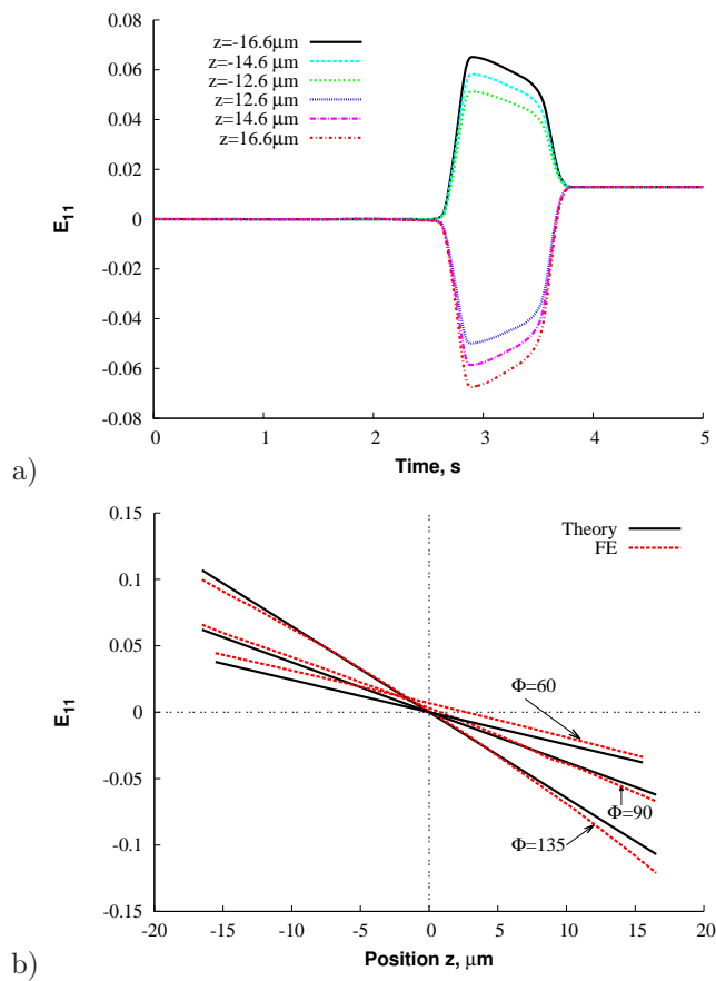
Figure 7: a) Time evolution of the longitudinal strain component E_{11} within the film thickness for the peel angle \Phi = 90 . b) Maximum through thickness longitudinal strain captured by the Finite element. Comparison with the bending approach for three peel angles : 60^\circ , 90^\circ and 135^\circ . Material parameters are those of Table 1 with \gamma = 40 .
