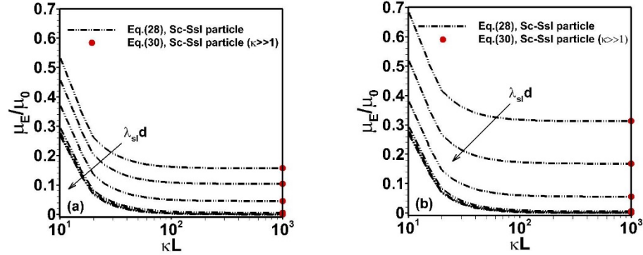
Fig. 3. Dependence of scaled electrophoretic mobility of Sc-Ssl particles obtained from Eq. (28) on dimensionless \kappa L at fixed L = 100 nm, d = 10 nm with \rho_{shell} / z_{shell} F = \rho_{core} / z_c F = 1 mM, (a) \lambda_c^{-1} = 1 nm, (b) \lambda_c^{-1} = 10 nm and for various values of \lambda_{sl}^{-1} ( = 0.1, 0.2, 0.5, 1, 2, 5, 10 nm) (growing \lambda_{sl} d values in the direction given by the arrows). For the sake of comparison, value of the electrophoretic mobility of Sc-Ssl particles in the limit of infinite electrolyte concentrations (Eq. (30)) is further reported (red dots).
