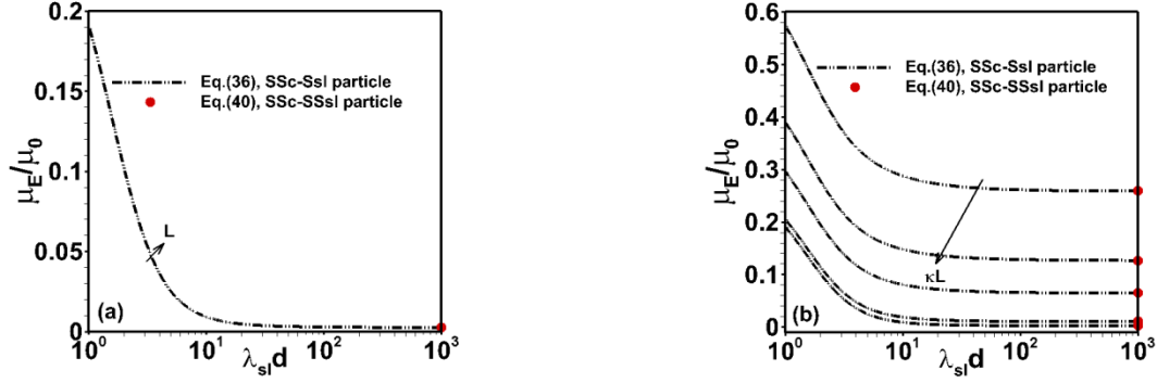
Fig. 5. Dependence of scaled electrophoretic mobility of SSc-Ssl particles obtained from Eq. (36) on dimensionless \lambda_{sl}d for d = 10 nm, with \rho_{shell}/z_{shell}F = \rho_{core}/z_cF = 1 mM. The results are shown for (a) \kappa^{-1} = 1 nm at various values of L = 10, 50, 100, 200, 500 nm (growing L values in the direction given by the arrow). In panel (b), results are given for various values of \kappa L at fixed L = 100 nm. For the sake of comparison, the value of the electrophoretic mobility of SSc-SSsl particles obtained from Eq. (40) is further reported (red dots).
