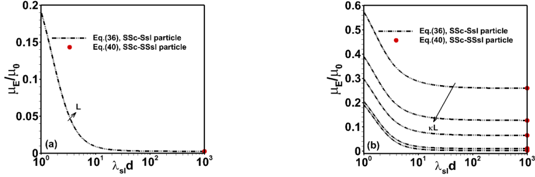
Fig. 5. Dependence of scaled electrophoretic mobility of SSc-Ssl particles obtained from Eq. (36) on dimensionless \lambda_{sl}d for d = 10 nm, with \rho_{shell} / z_{shell}F = \rho_{core} / z_cF = 1 mM. The results are shown for (a) \kappa^{-1} = 1 nm at various values of L = 10, 50, 100, 200, 500 nm (growing L values in the direction given by the arrow). In panel (b), results are given for various values of \kappa L at fixed L = 100 nm. For the sake of comparison, the value of the electrophoretic mobility of SSc-SSsl particles obtained from Eq. (40) is further reported (red dots).
