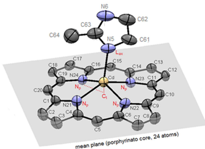
Figure 2. Distorted square pyramidal coordination geometry for complex I , showing the atom labelling. H atoms and meso groups are omitted for clarity and only the major position of the 2-MeHIm axial ligand is shown.
