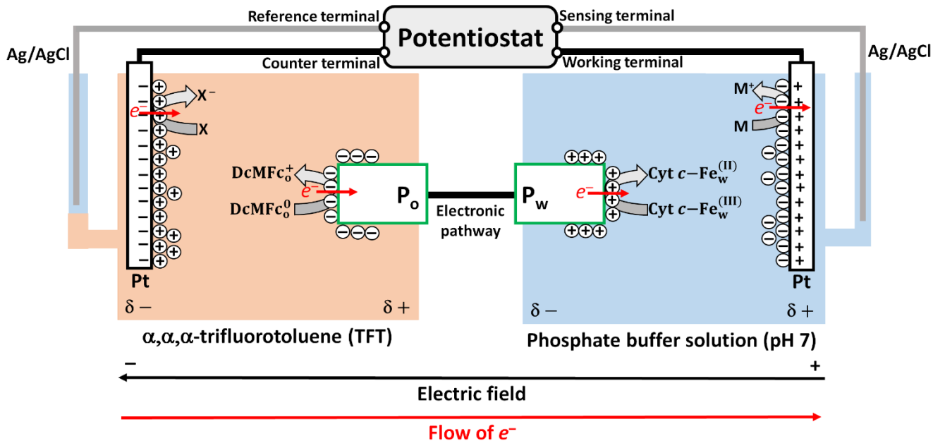
Scheme 2. Schematic of the 4-electrode CBPEC configuration with aqueous-organic electrolyte solutions used for the study of Cyt c bioelectrochemistry as \Delta_o^w \phi is biased sufficiently positively by the potentiostat to facilitate electron transfer along the BPE from the organic electron donor DcMFC at P_o to the aqueous Cyt c molecule at P_w .
